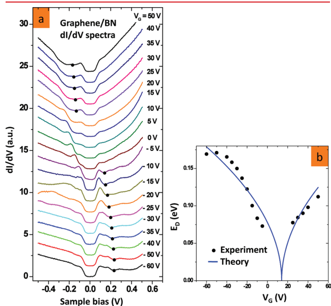
Figure 3. Gate dependence of differential conductance ( dI/dV ) spectra. (a) Typical STM dI/dV spectra of graphene/BN obtained with tunnel junction impedance = 2.5 GΩ (set point: I_T = 0.2 nA, V_b = -0.5 V). Black dots mark minima in spectra used to extract the Dirac point energy (see text). (b) Black dots: Dirac point energy vs gate voltage extracted from dI/dV spectra (see text). The blue curve is a theoretical fit using the square-root dependence of the Dirac point energy vs gate voltage.
