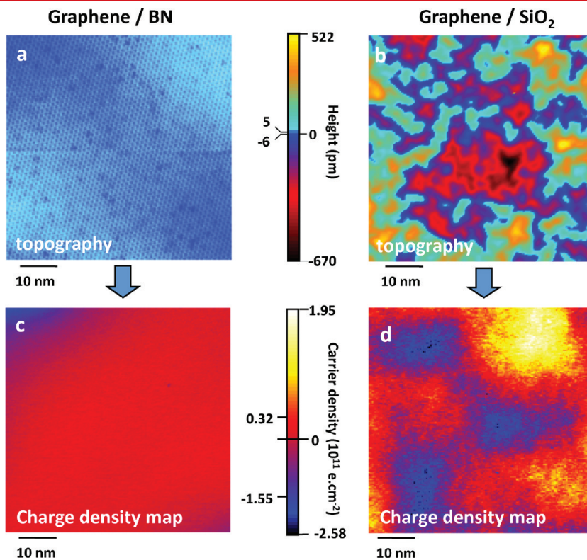
Figure 4. Comparing topography and charge density for graphene/BN vs graphene/SiO 2 . (a,b) The 60 nm × 60 nm STM topographs of (a) graphene/BN ( I_T = 0.2 nA, V_b = 0.25 V, V_G = -6 V) and (b) graphene/SiO 2 ( I_T = 0.02 nA, V_b = -0.225 V, V_G = 15 V). Charge density maps obtained from conductance maps (see text) are shown for (c) graphene/BN (same area as in (a), acquired simultaneously) and (d) graphene/SiO 2 (same area as in (b), acquired simultaneously). The minima and maxima marked in the scales are the minima and maxima of the respective images.
