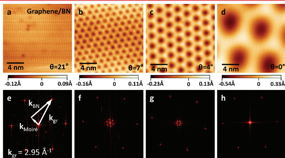
Figure 2. Graphene/BN surface topography. (a–d) The 20\text{ nm} \times 20\text{ nm} constant current STM topographs at four different graphene/BN locations show how the graphene/BN Moiré pattern changes depending on the rotational orientation ( \theta ) between graphene and the BN lattices (see text). (a) I_T = 0.1 nA, V_b = 0.15 V, V_G = -25 V, \theta = 21 \pm 1^\circ . (b) I_T = 0.2 nA, V_b = 0.15 V, V_G = 0 V, \theta = 7 \pm 1^\circ . (c) I_T = 0.2 nA, V_b = 0.15 V, V_G = -6 V, \theta = 4 \pm 1^\circ . (d) I_T = 0.15 nA, V_b = 0.15 V, V_G = -3 V, \theta = 0 \pm 1^\circ . (e–h) Fourier transforms of the topographs (a–d). The outer spots show the graphene reciprocal lattice, the inner spots show the graphene/BN Moiré pattern reciprocal lattice.
