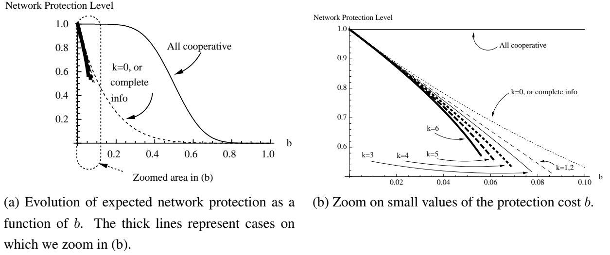
Figure 3: Weakest link. Evolution of the network protection level as a function of the protection cost b . The short lines illustrate the presence of limiting conditions on protection equilibria for this game. Where the lines end, the expected network protection level becomes zero. Also note that the cases k = 1 and k = 2 produce identical curves.
