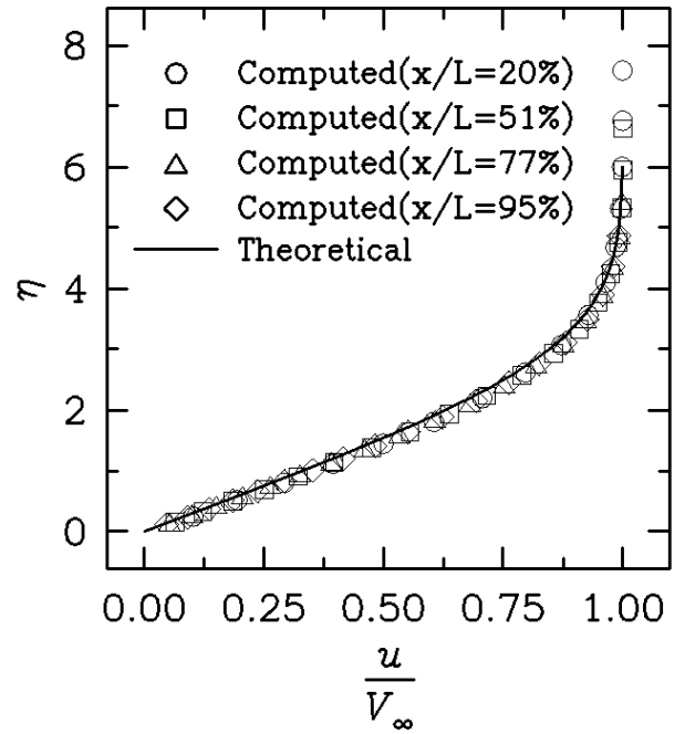
Fig. 4 Comparison of exact Blasius solution for laminar flow over flat plate with USM3Dns result. M_\infty=0.5 , Re_L=10000 .
