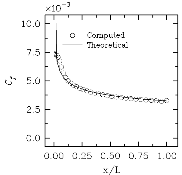
Fig. 5 Comparison of computed vs. theoretical skin friction coefficient for turbulent flat-plate flow. M_\infty=0.5 , Re_L=2 million.
