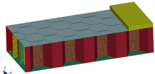
Fig. 7 Honeycomb ribbon orientation parallel to span of sandwich beam-detailed model
