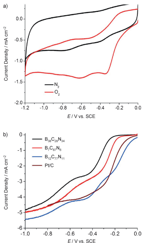
Figure 3. a) Cyclic voltammetry (CV) curves of ORR on BCN ( B_{12}C_{77}N_{11} ) graphene in nitrogen- and oxygen-saturated 0.1 M KOH solutions at a scan rate of 50 \text{ mV s}^{-1} . b) LSV curves of ORR on BCN graphene with different compositions in oxygen-saturated 0.1 M KOH solution at 10 \text{ mV s}^{-1} and compared with the commercial Pt/C electrocatalyst.
