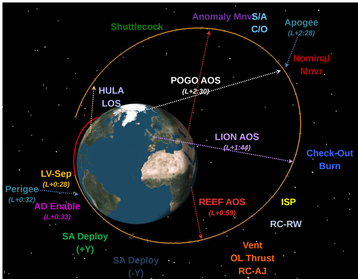
Figure 6. TacSat-4 First Orbit Overview
