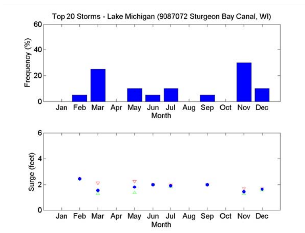
Figure 60. PDS surge values by month for Sturgeon Bay gage.
