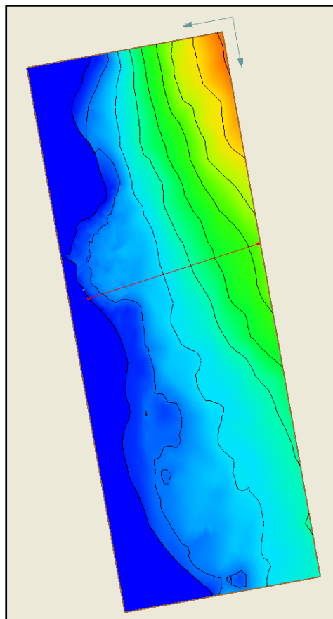
Figure 74. CMS-Wave grid extents, bathymetry and beach transect.
