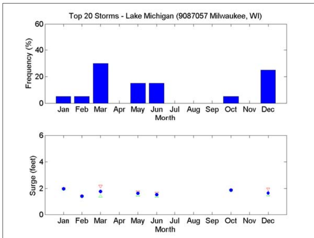
Figure 58. PDS surge values by month for Milwaukee gage.
