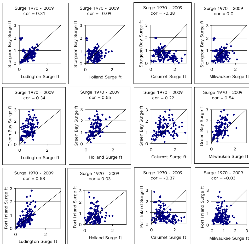
Figure 53. Measured surge correlations between gages.
