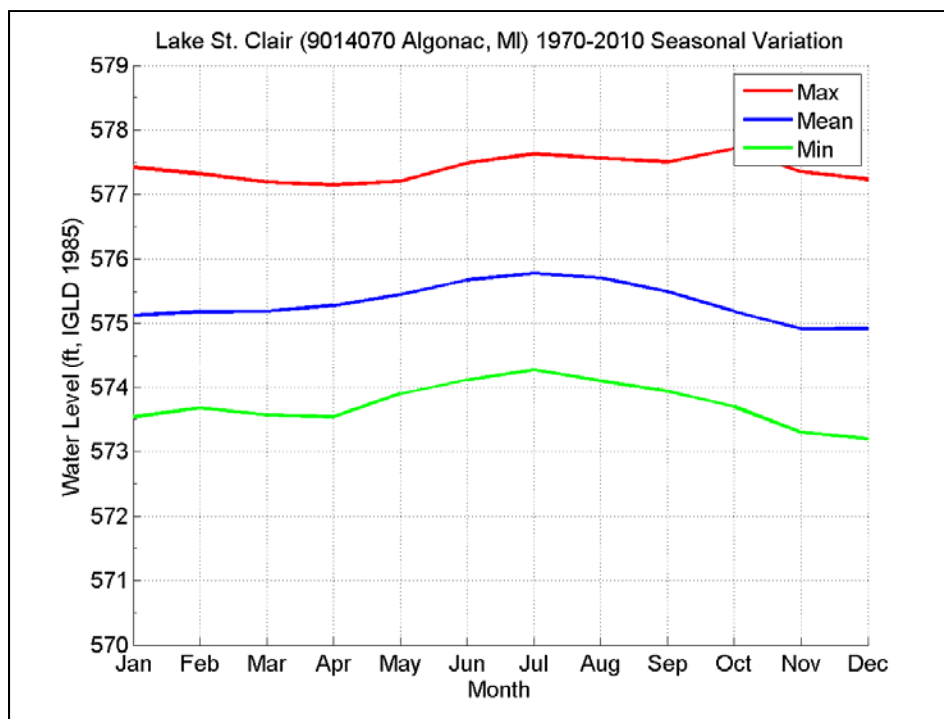
Figure 38. Algonac mean and extremes of measured water levels during the period 1970 – 2010.
