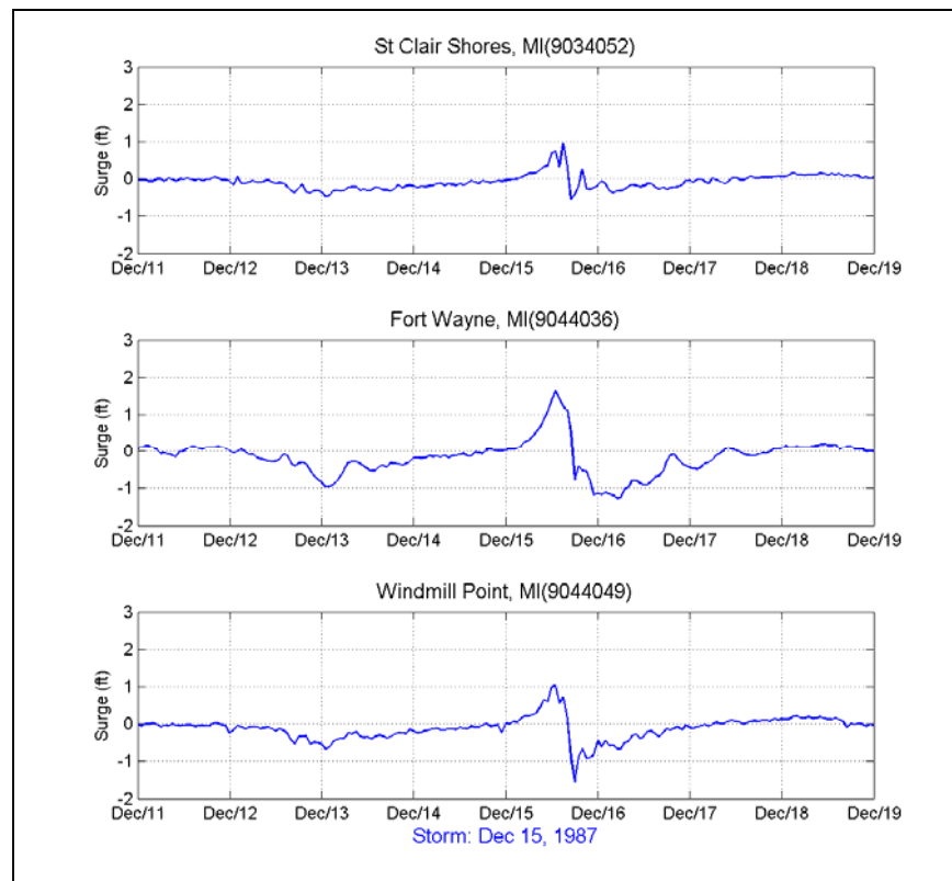
Figure C10. Surge measurements at each gage station during the event.
