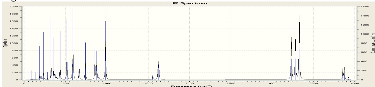
Figure 4. IR intensity as a function of frequency calculated using DFT for Mg-3H2O-1O3a, Mg2-3H2O-1O3b, Mg-3H2O-1O3b, Mg-3H2O-1O3c and Mg-3H2O-1O3d according to frozen phonon approximation.
