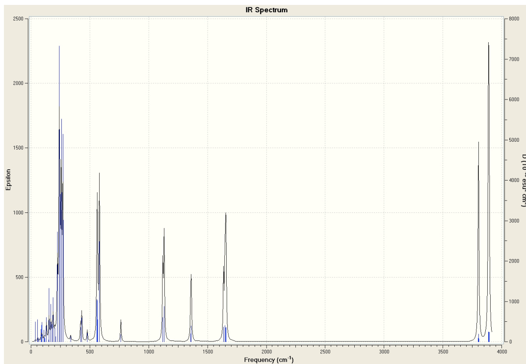
Figure 9F. IR intensity as a function of frequency calculated using DFT for Mg-4H 2 O-2O 3 c1 in water solvent according to frozen phonon approximation.
