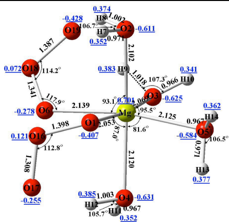
Mg2-4H2O-2O3c1
