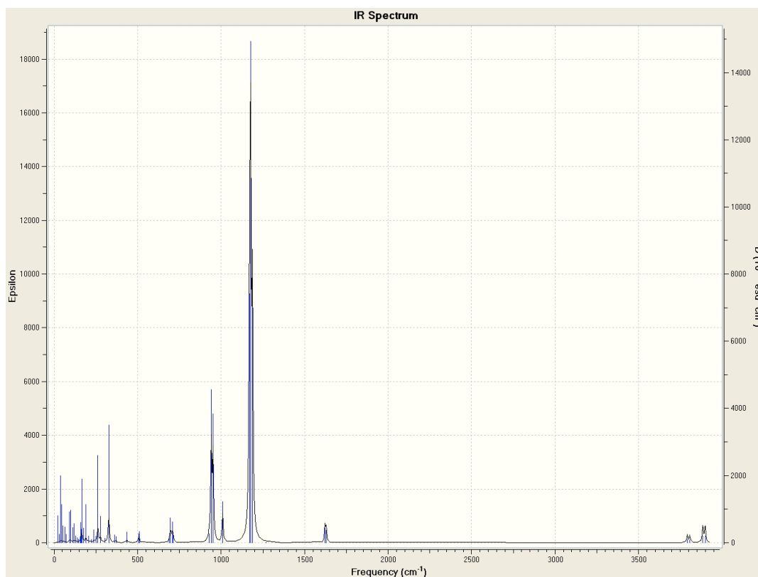
Figure 9C. IR intensity as a function of frequency calculated using DFT for Mg 2 -2H 2 O-4O 3 c in water solvent according to frozen phonon approximation.
