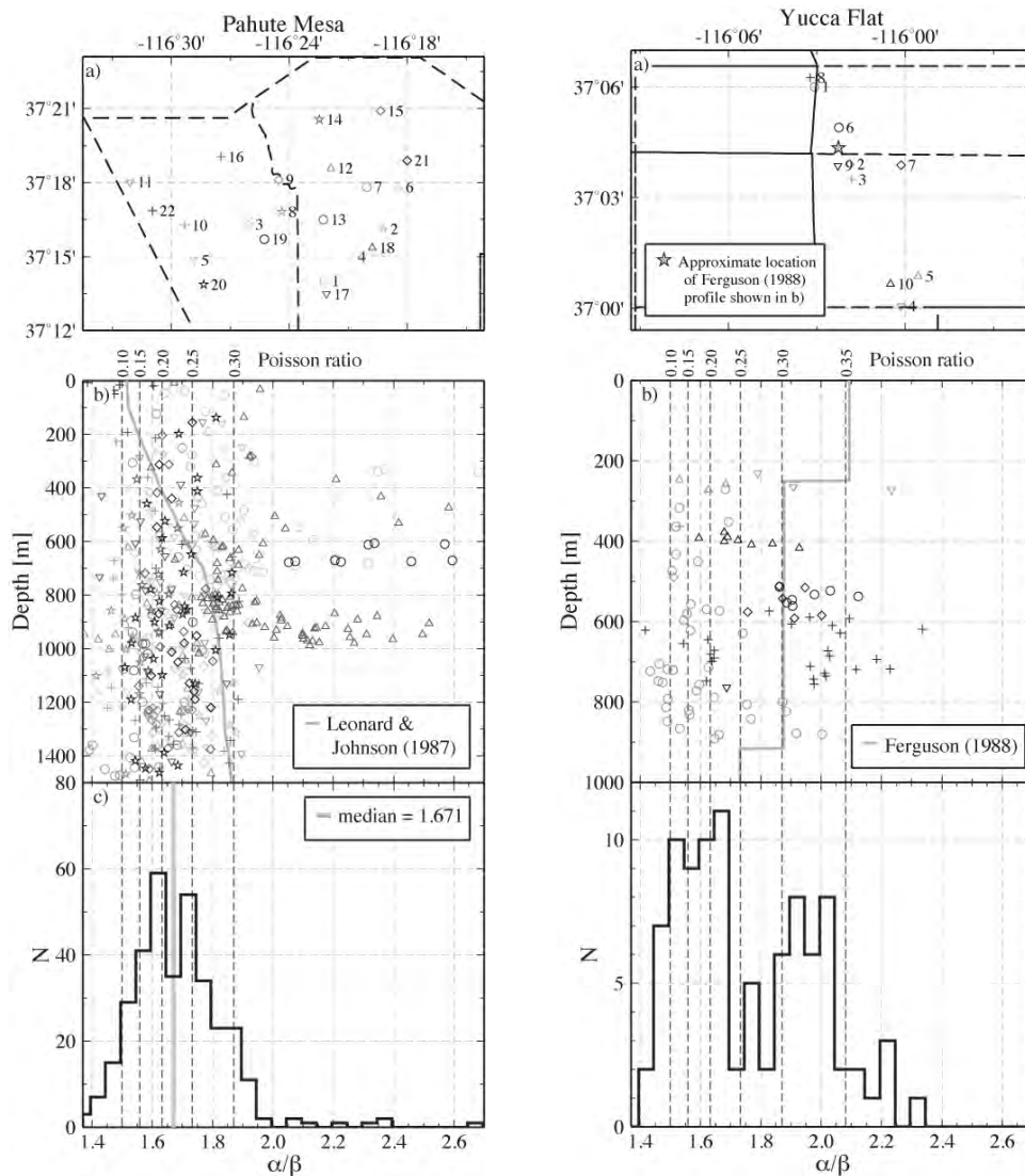
Figure 6. Analysis of V_p/V_s ( \alpha/\beta ) ratio from USGS database (Wood, 2007) at Pahute Mesa and Yucca Flat. The ratio as a function of depth from Leonard and Johnson (1987) and Ferguson (1988) are shown for Pahute Mesa and Yucca Flat, respectively. Based on the distribution, we estimate constant V_p/V_s ratios of 1.671 and 1.871 ( \nu = 0.3 ) at Pahute Mesa and Yucca Flat, respectively.
