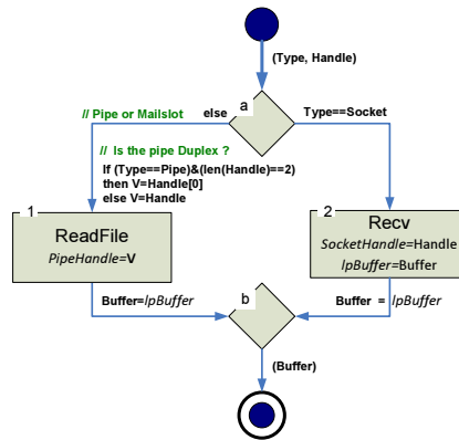
Figure B-2. Remote IPC – Receive Operation
