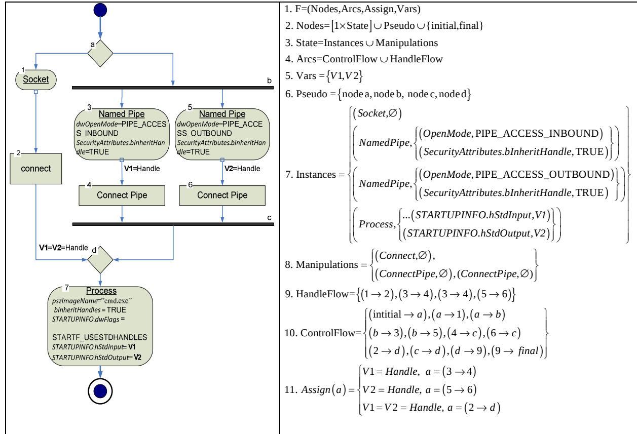
Figure 6. Activity Diagram of the “Remote Shell” Functionality
