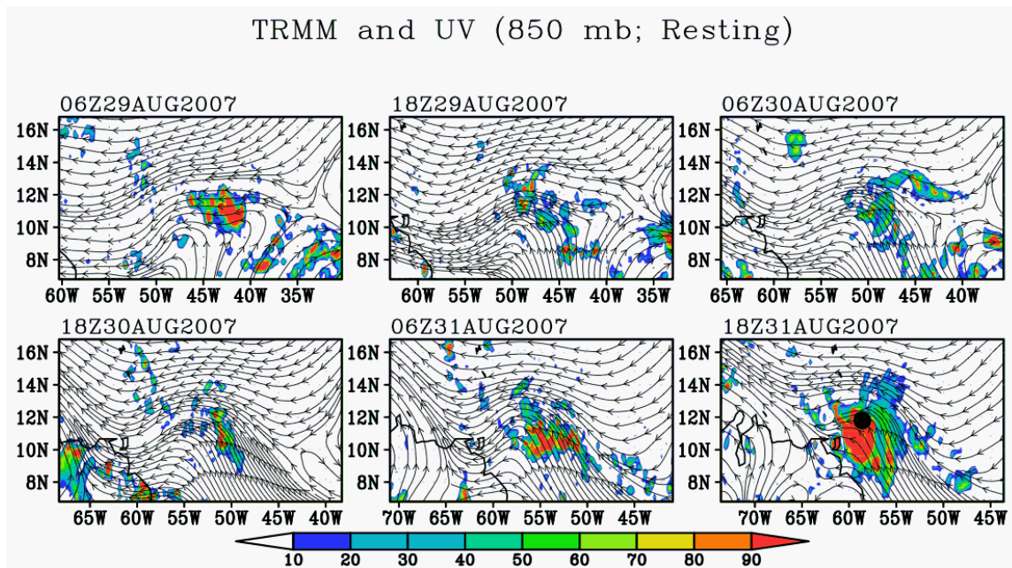
Figure 3. Streamlines of the 2.5-day low-pass filtered 850-hPa flow from ECMWF analyses in the Earth-relative frame of reference from 0600 UTC 29 Aug to 1800 UTC 31 Aug. Shading indicates TRMM 3-h accumulated precipitation ( \text{mm day}^{-1} ). The genesis location is indicated by the black dot in the final panel.
