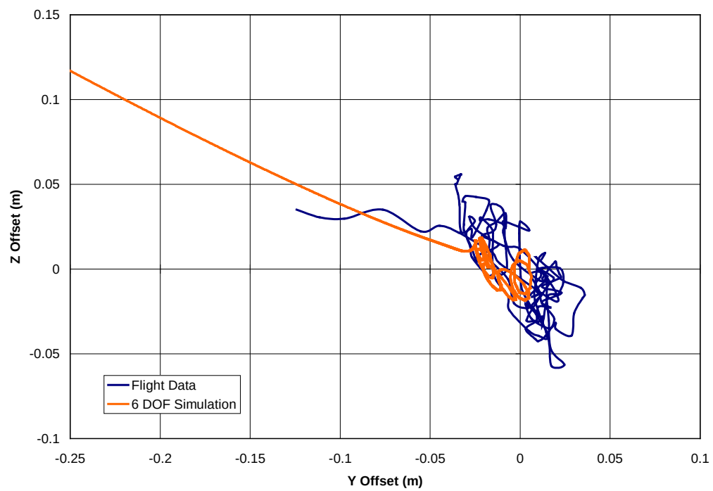
Figure 8.9. Simulation vs. trajectory data in the Y-Z plane for Flight 1.
