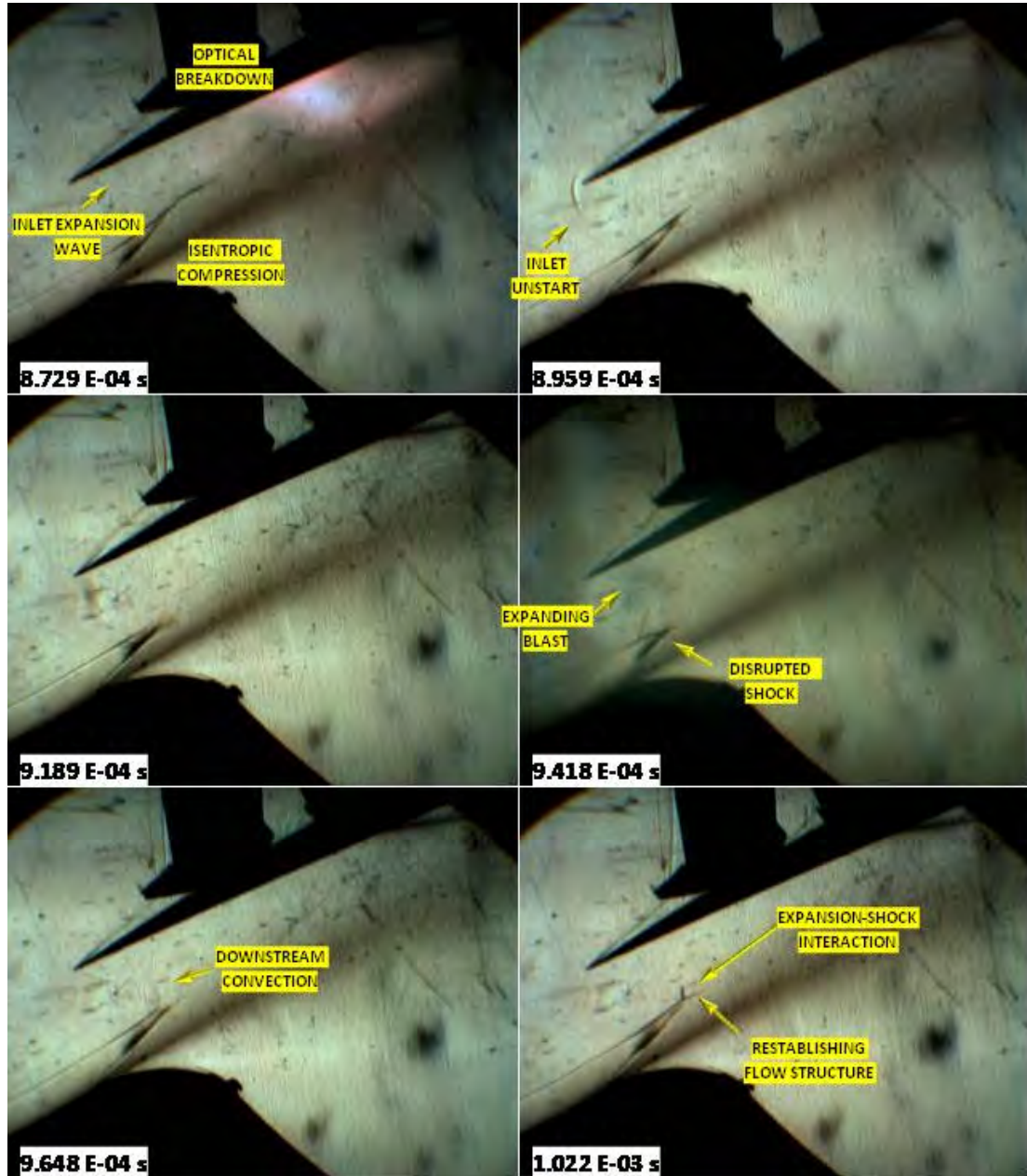
Figure 5.26: Run#23 - Laser induced blast wave interaction with oblique shocks and shroud under-surface. Model at -7.5^\circ and shroud at -24^\circ inclination. ( M=9.43 , T_\infty=113.7 \text{ K} , P_\infty=0.293 \text{ kPa} , E_p=106\pm11 \text{ J} )
