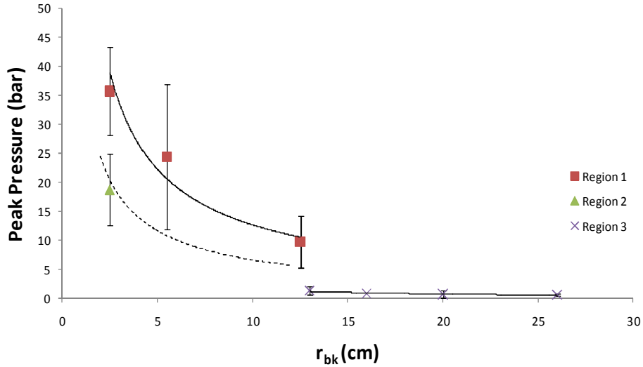
Figure 1.16: Run #12—Peak surface pressure vs. distance from laser focal line. ( P_{\infty} = 1 bar; E_p = 180 ± 20 J)
