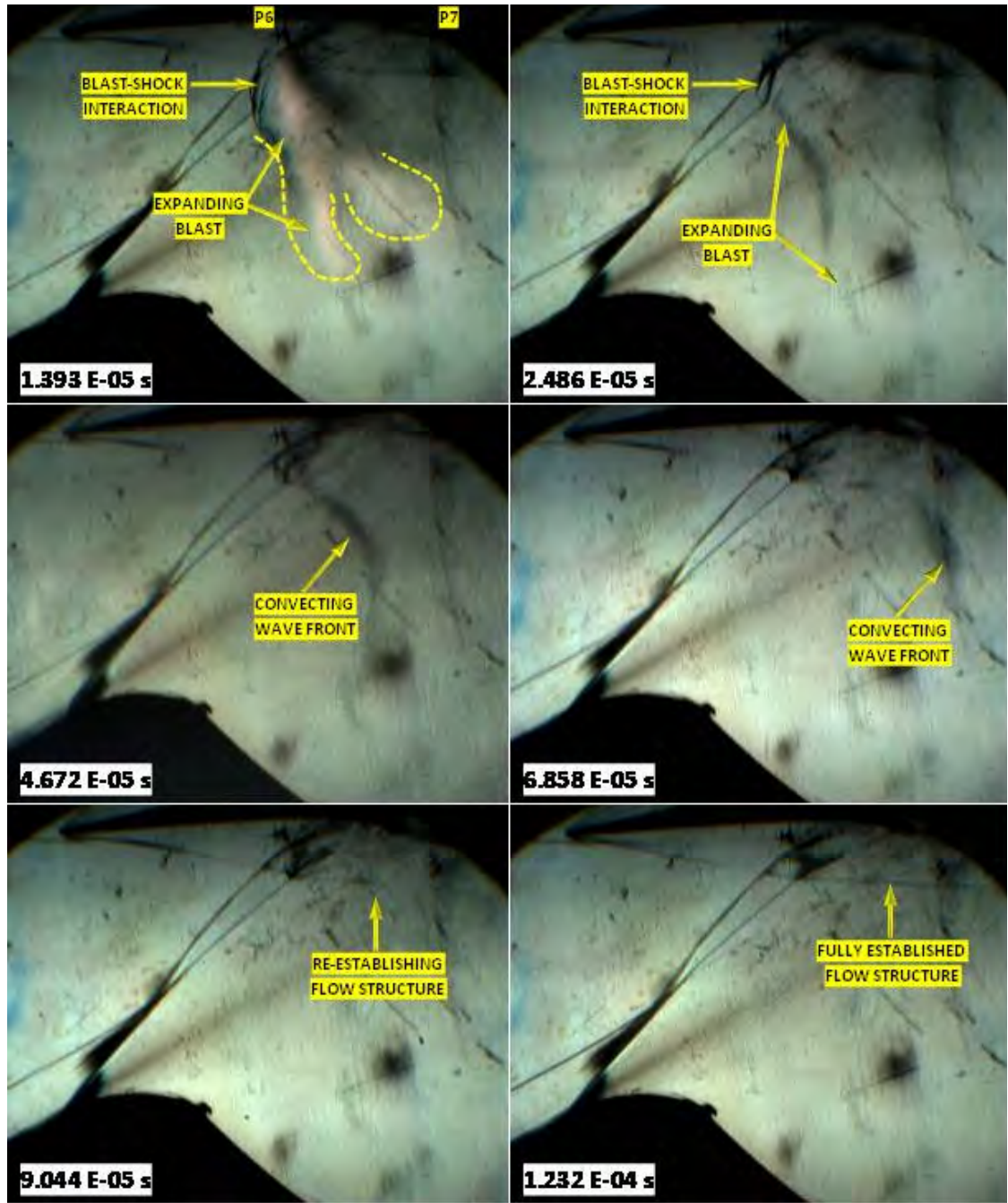
Figure 5.15: Run#17 - Laser induced blast wave interaction with oblique shocks and shroud under-surface; 2D model at -7.5^\circ ; Shroud at -4^\circ inclination. ( M=5.94 , T_\infty=256.8 \text{ K} , P_\infty=6.25 \text{ kPa} , E_p=186\pm 19 \text{ J} )
