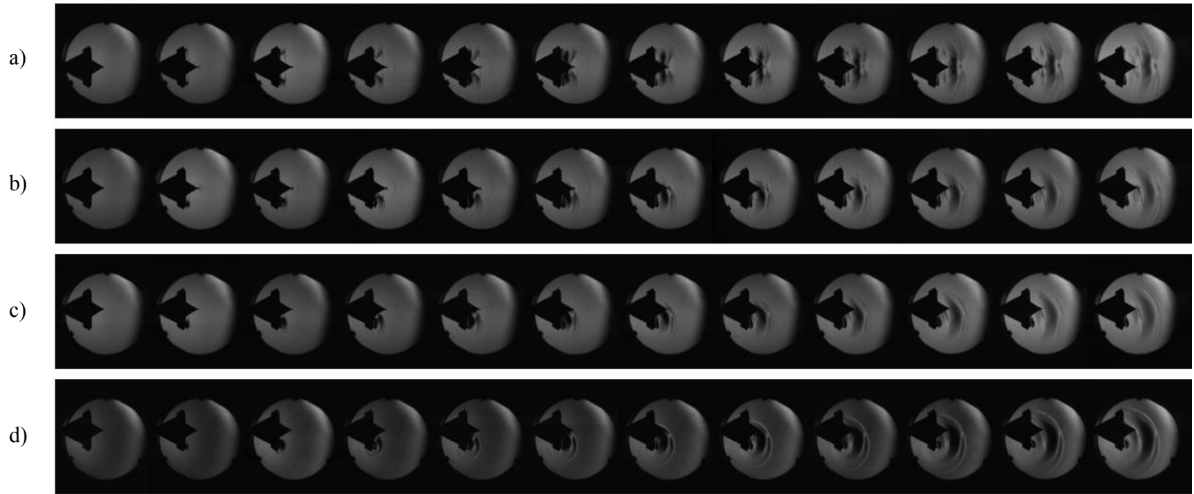
Figure 4.16. Schlieren photography of #200-2/3 with laser offset downward from engine centerline by: a) 0% D_e , b) 10% D_e , c) 20% D_e , d) 30% D_e . (~13 J pulse, ~20.5 \mu s step).
