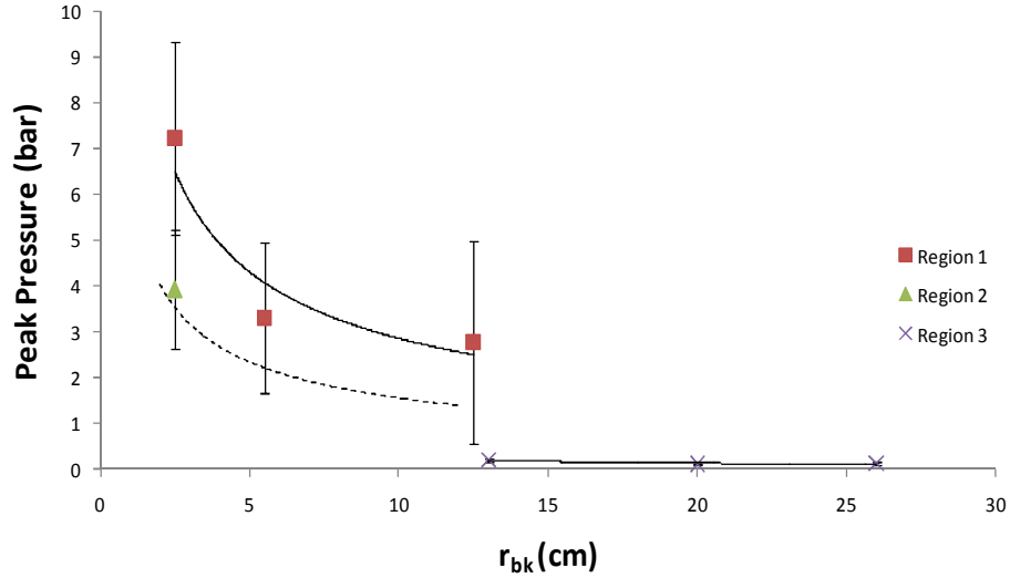
Figure 1.15: Run #11—Peak surface pressure vs. distance from laser focal line. ( P_{\infty} = 300 mbar; E_p = 231 ± 23 J)
