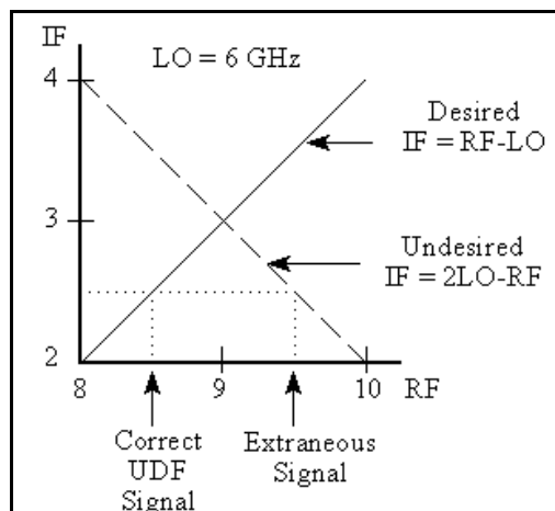
Figure 5. Low Side Mixing Results
