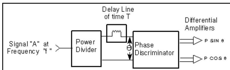
Figure 2. Frequency Discriminator
