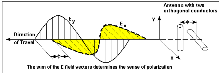
Figure1. Polarization Coordinates
