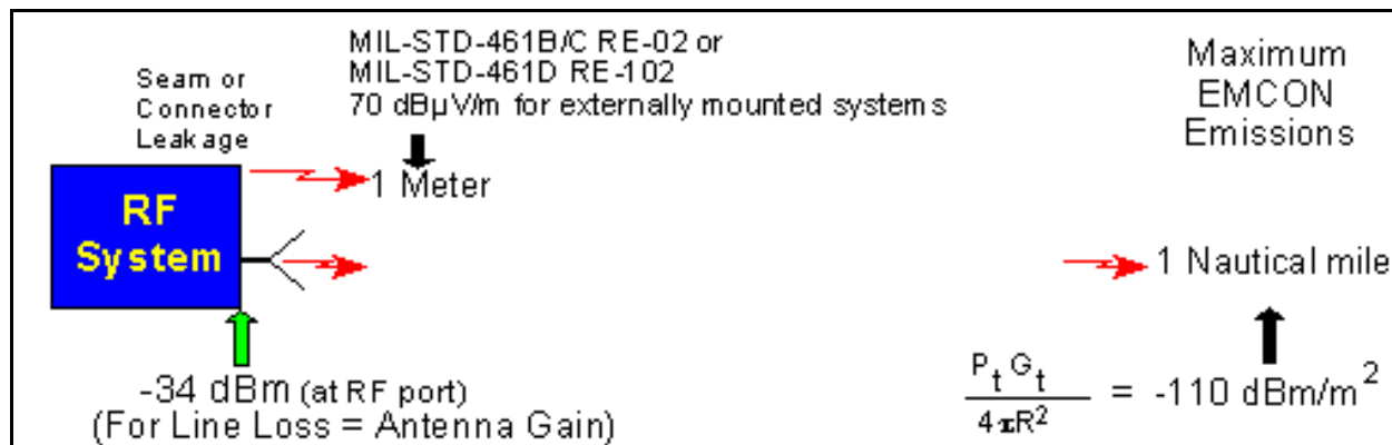
Figure 1. EMCON Field Intensity / Power Density Measurements
