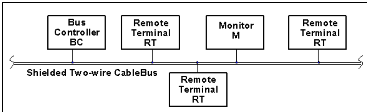
Figure 1. 1553 Bus Structure
