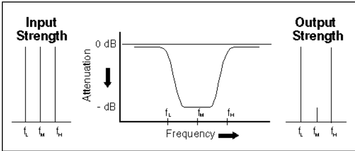
Figure 4. Band-Reject Filter
