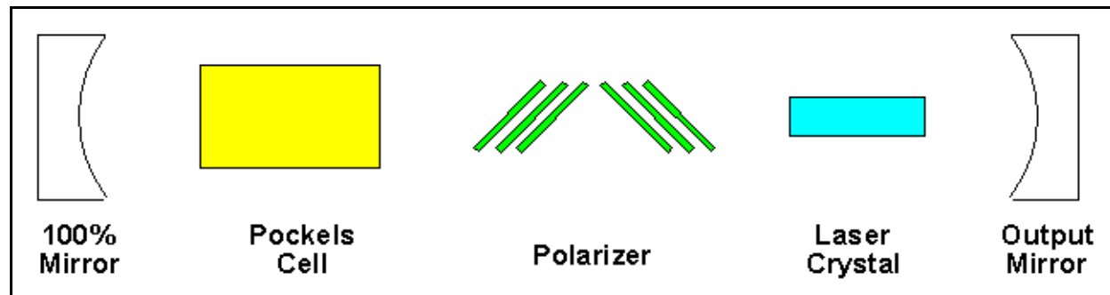
Figure 39. Q-Switch Arrangement
