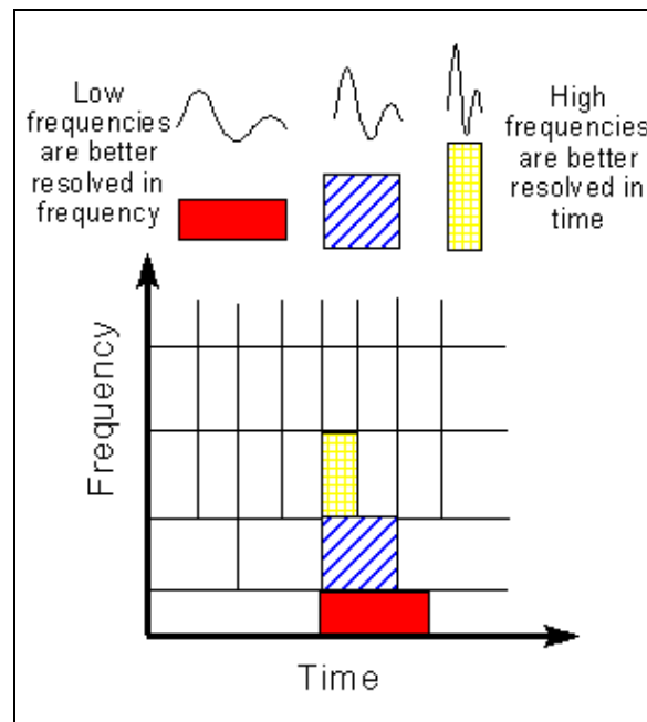
Figure 6. Wavelet Transform
