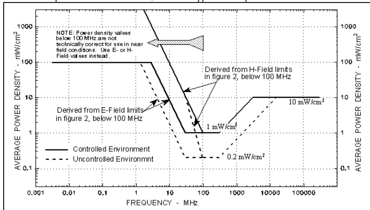
Figure 3. Radiation Hazards to Personnel from DoD INST 6055.11
