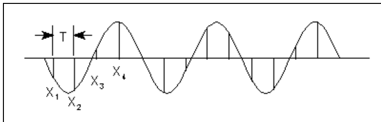
Figure 2. Waveform Sampling
