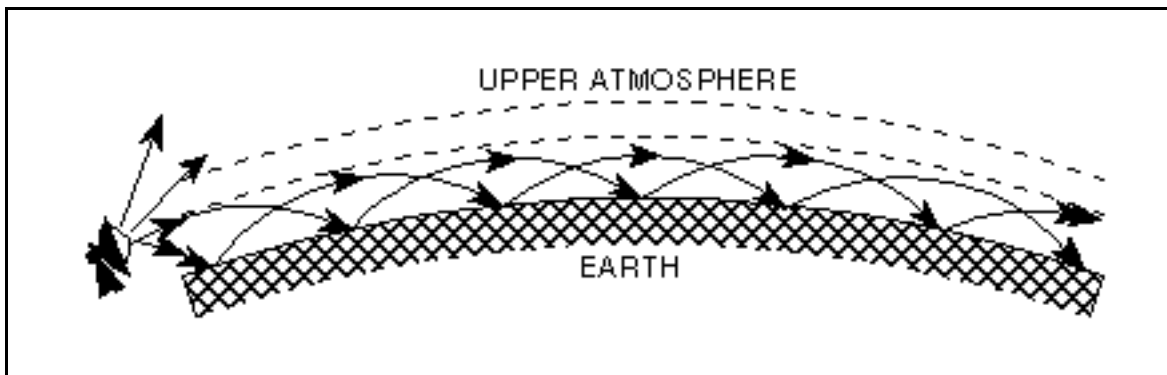
Figure 3. Ducting
