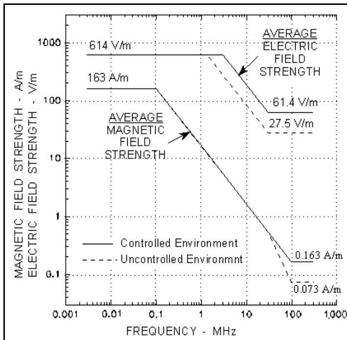
Figure 2. Lower Frequency HERP from DoD INST 6055.11
