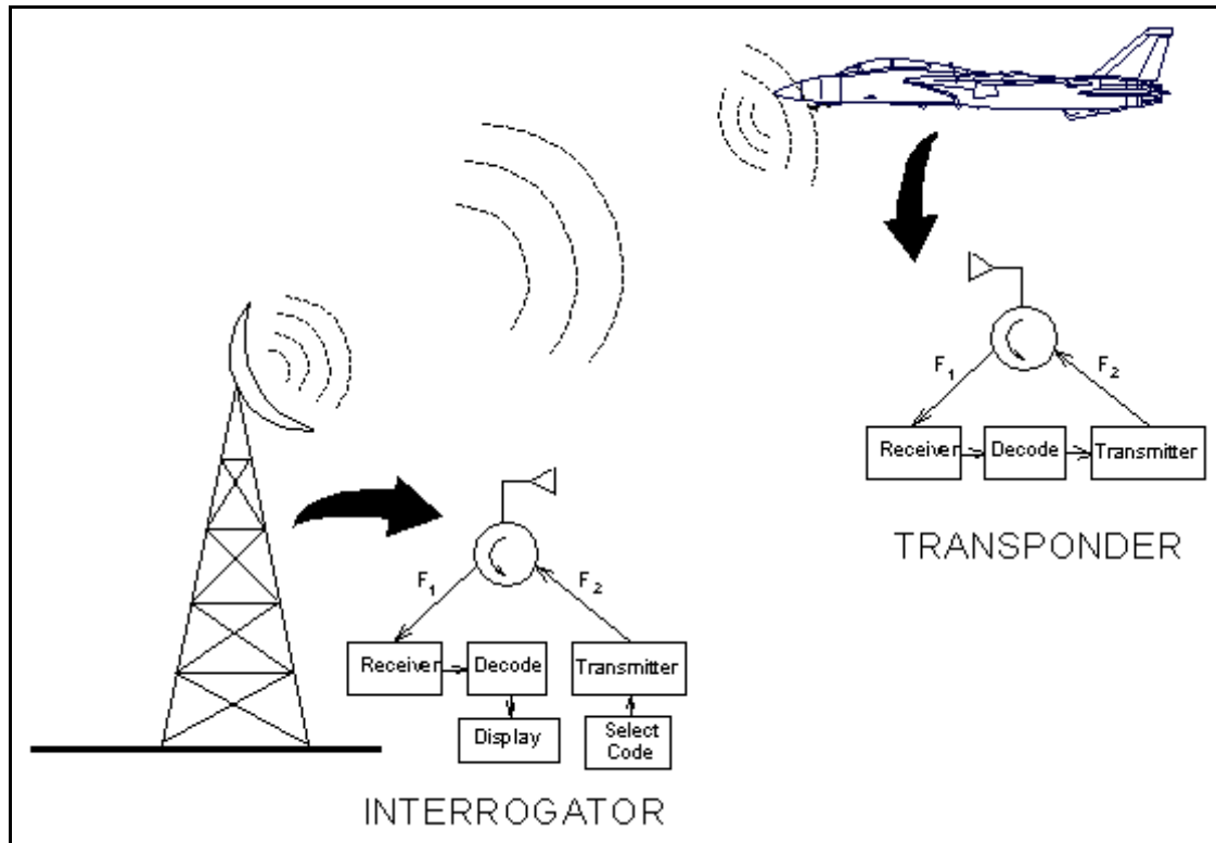
Figure 1. IFF Transponder
