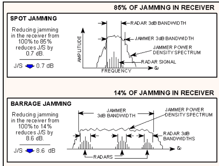
Figure 2. Noise Jamming
