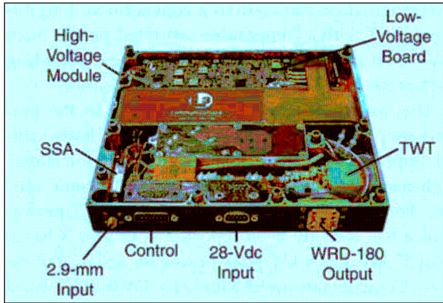
Figure 3: 40W Ka-band MPM with components identified.
