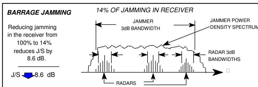
Figure 2. Barrage Jamming
