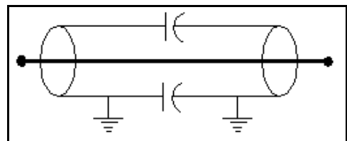
Figure 6. Outside DC Block
