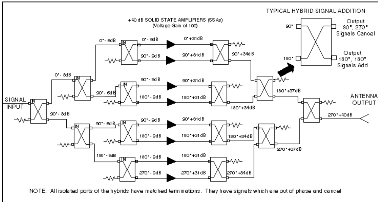
Figure 6. Combiner Network
