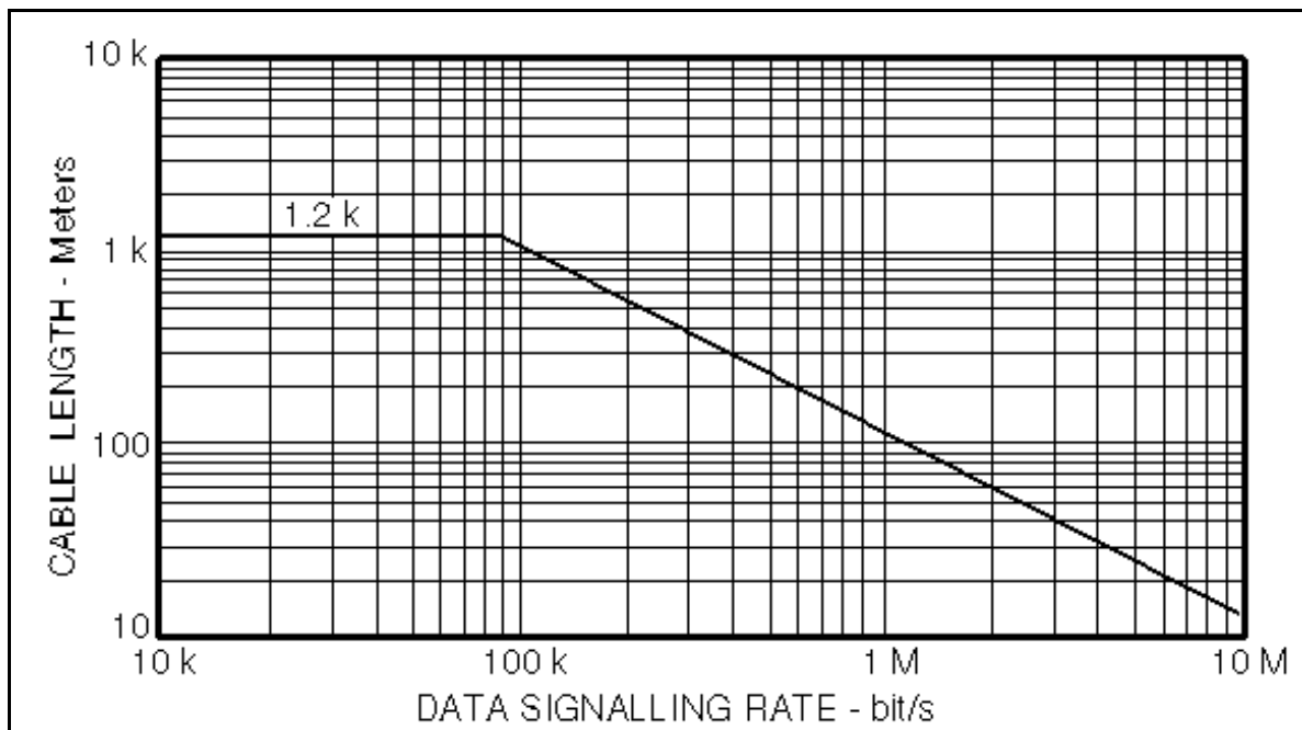
Figure 3. Data Signaling Rate vs Cable Length
