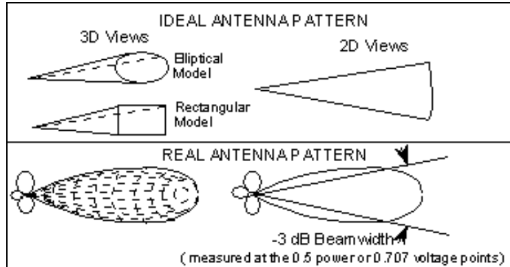
Figure 3. Antenna Beamwidth
