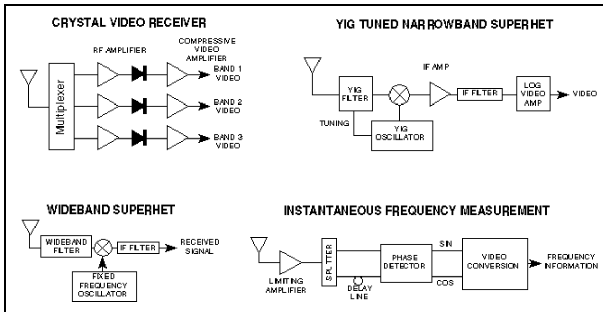
Figure 1. Common ESM Receiver Block Diagrams
