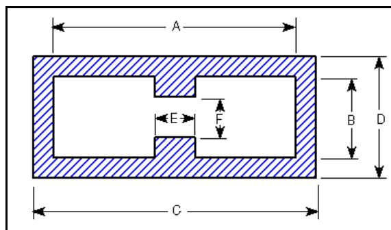
Figure 3. Double Ridge Waveguide
