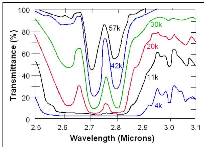
Figure 13. Transmittance at Various Altitudes
