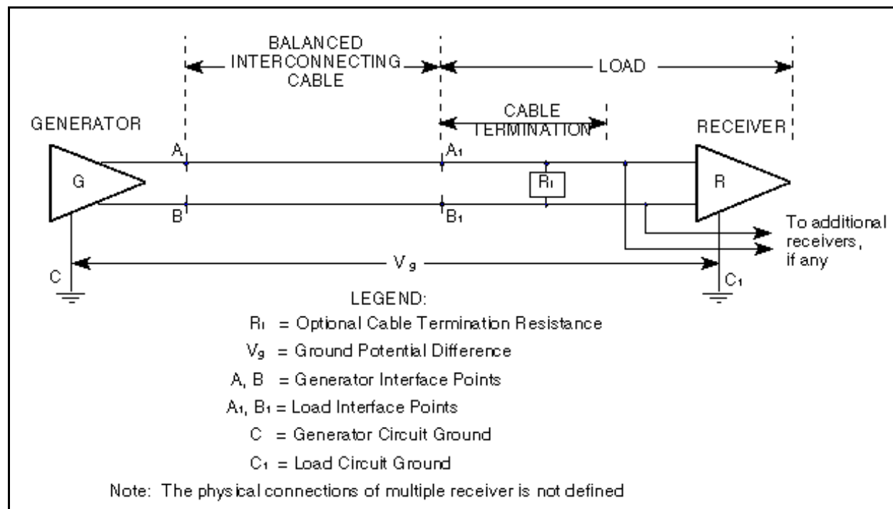
Figure 2. Balanced Digital Interface Circuit
