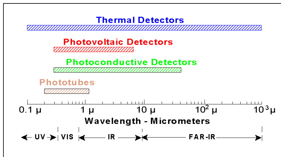
Figure 18. Spectral Range of Various Detectors
