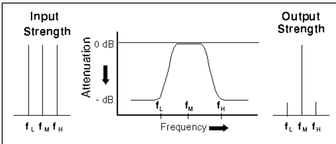
Figure 3. Band-Pass Filter
