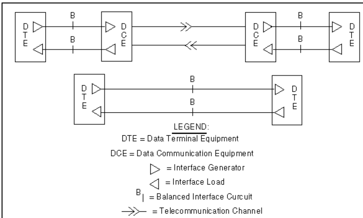
Figure 1. Application of a RS-422 Circuit
