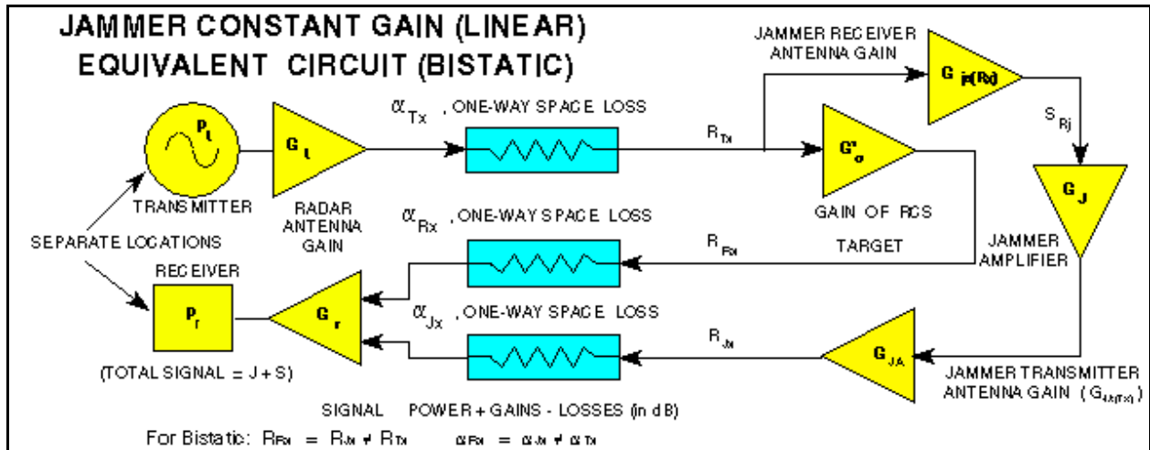
Figure 3. Jammer Constant Gain EA Equivalent Circuit (Bistatic)
