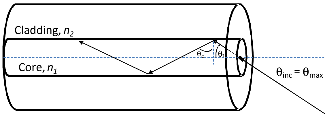
Figure 40. Bare Fiber Optic Cable
