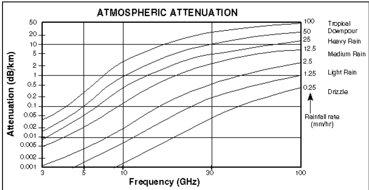
Figure 2. Atmospheric Attenuation
