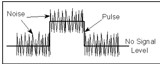
Figure 6. Tangential Sensitivity
