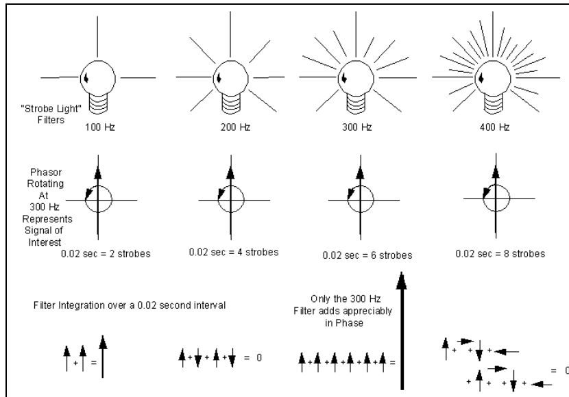
Figure 4. Phasor Representation
