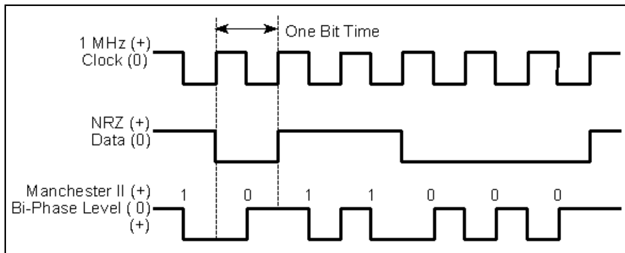
Figure 2. Data Encoding
