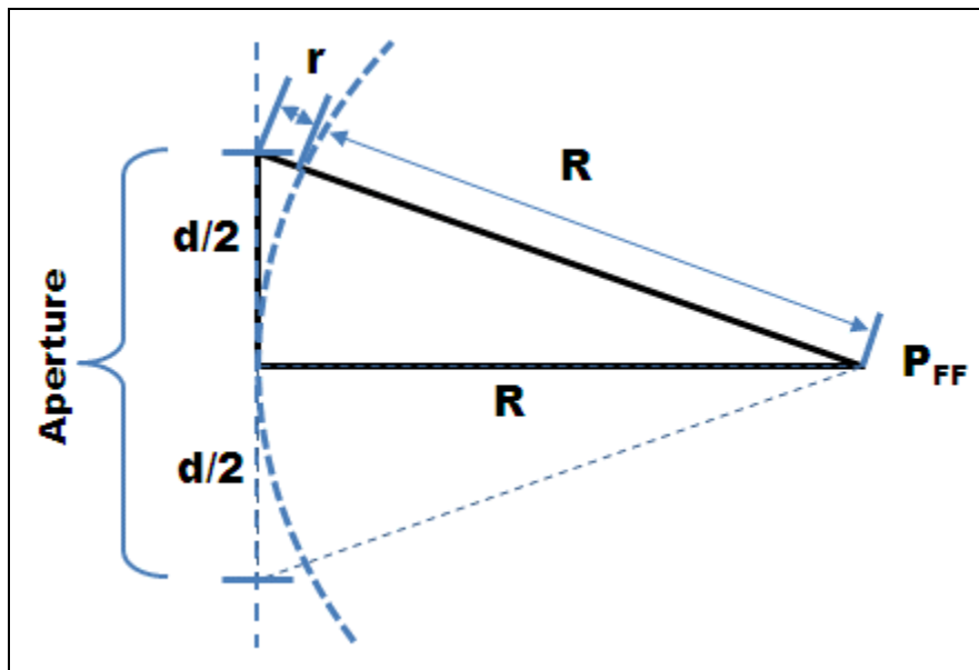
Figure 4. Alternative geometry for Far Field Estimation
