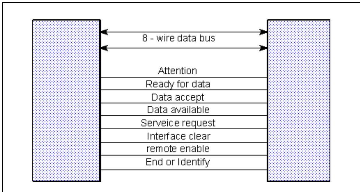
Figure 1. IEEE-488 (HP-IB / GP-IB) Bus Configuration
