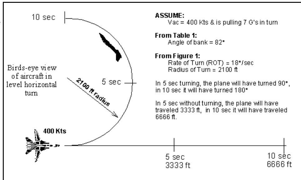
Figure 2. Maneuvering Aircraft
