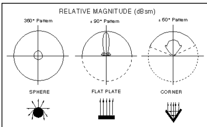
Figure 4. RCS Patterns
