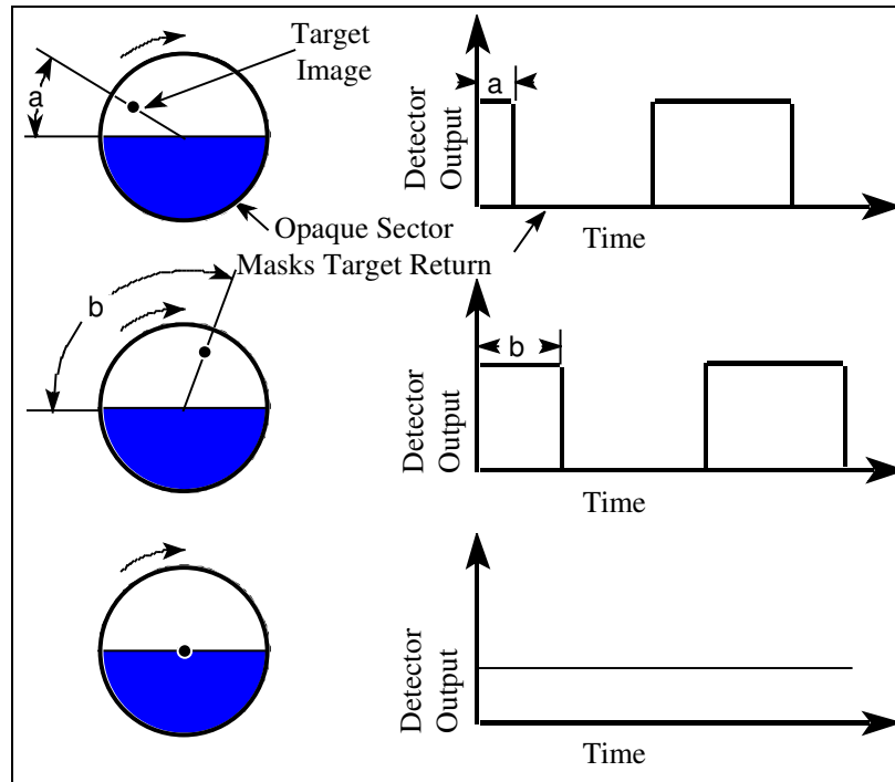
Figure 27. Basic Reticule Design
