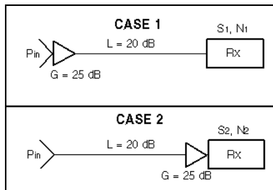
Figure 4. Pre-Amp S/N
