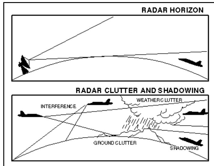
Figure 1. Radar Horizon and Shadowing
