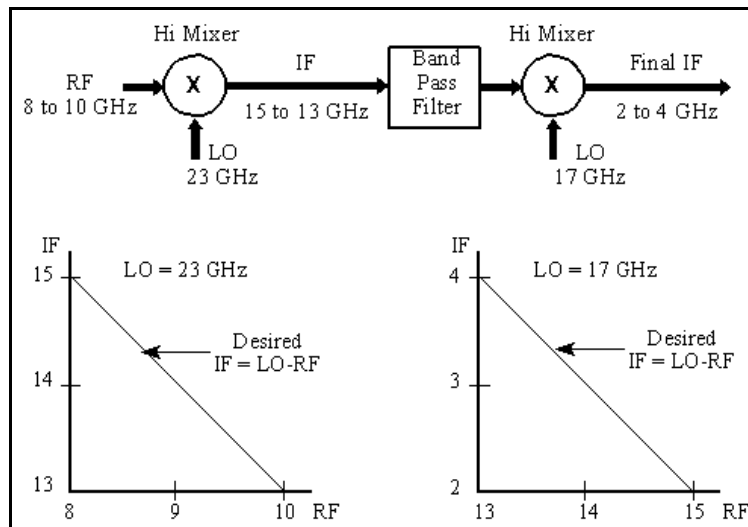
Figure 8. Double Mixing
