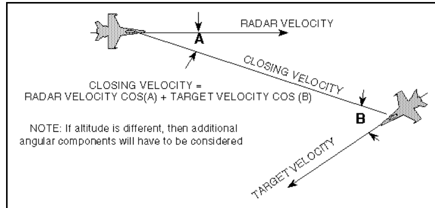
Figure 4. Doppler Depends Upon Closing Velocity
