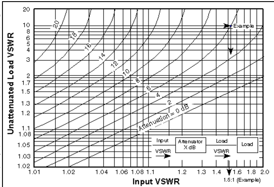
Figure 1. Reduction of VSWR by Attenuation
