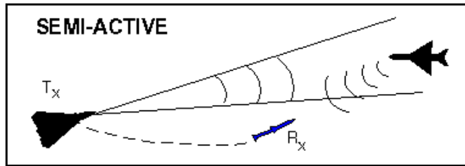
Figure 5. Bistatic Radar
