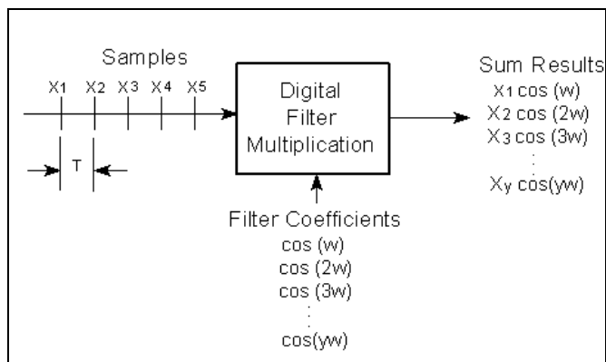
Figure 3. Digital Filtering
