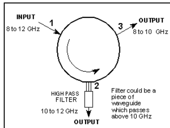
Figure 3. Diplexer From A Circulator
