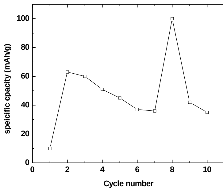
Fig 21: Variation of specific capacity of Li-air cell employing ionic liquid as a solvent. Cell area: 1.1 \text{ cm}^2 and current: 0.1 mA
