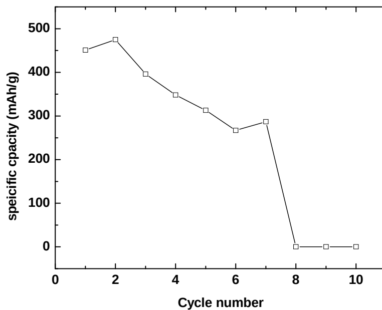
Fig 22: Variation of specific capacity of Li-air cell employing ether as a solvent. Cell area: 1.1 \text{ cm}^2 and current: 0.2 mA
