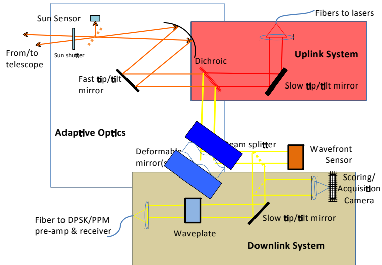
Figure 3 - Schematic of the integrated optical system to be located at coudé focus in OCTL
