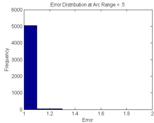
Figure 31. Error Distribution
