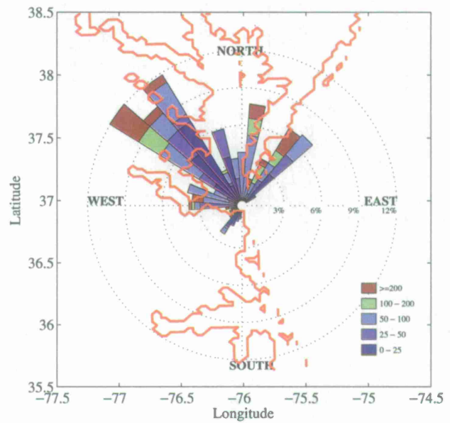
Fig. 25 A wind rose located at Cape Henry for 12–14 June 2010 depicting frequency of occurrence (in percent) and magnitude of the current error (color). The shoreline from the 3-km COAMPS is depicted in red
