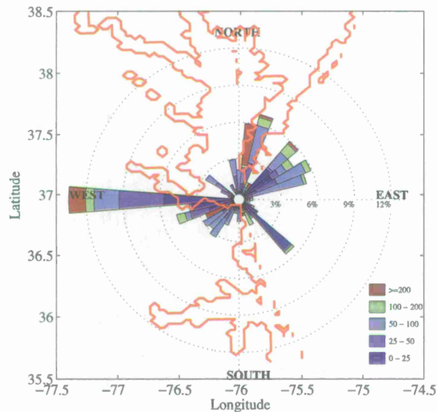
Fig. 24 A wind rose located at Cape Henry for 10–12 June 2010 depicting frequency of occurrence (in percent) and magnitude of the current error (color). The shoreline from the 3-km COAMPS is depicted in red
