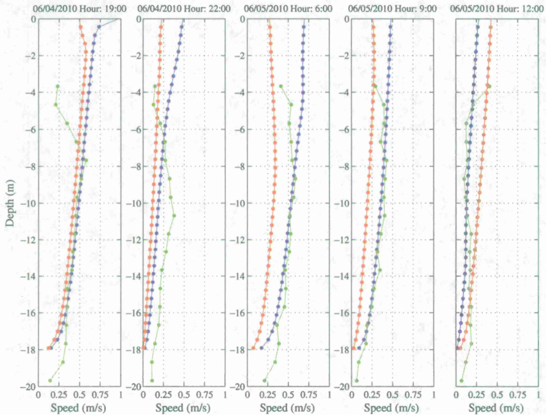
Fig. 20 Magnitude of the horizontal current modeled using 3-km winds (blue) and 27-km winds (red) vs. the observed values (green) on 4 June 2010 at 1900 hours and 2200 hours and on 5 June 2010 at 0600 hours, 0900 hours, and 1200 hours
