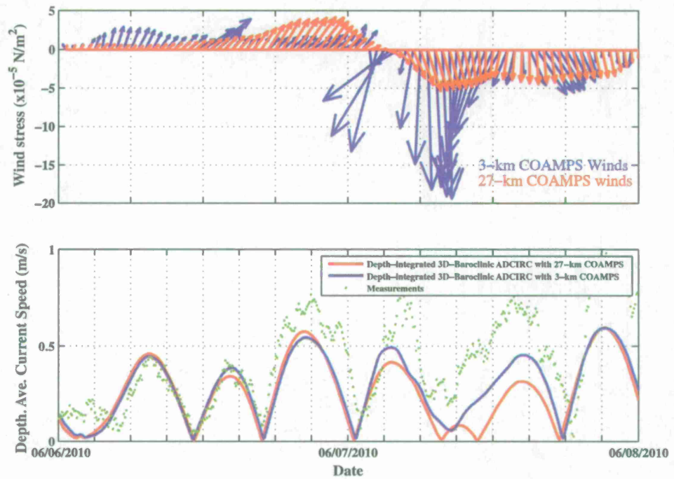
Fig. 16 Two-day model forecasts of baroclinic currents compared to observed currents (green) (both depth-averaged) from 6 to 8 June 2010 together with the applied COAMPS wind magnitude and direction from the 27-km (red) and 3-km (blue) resolution products
