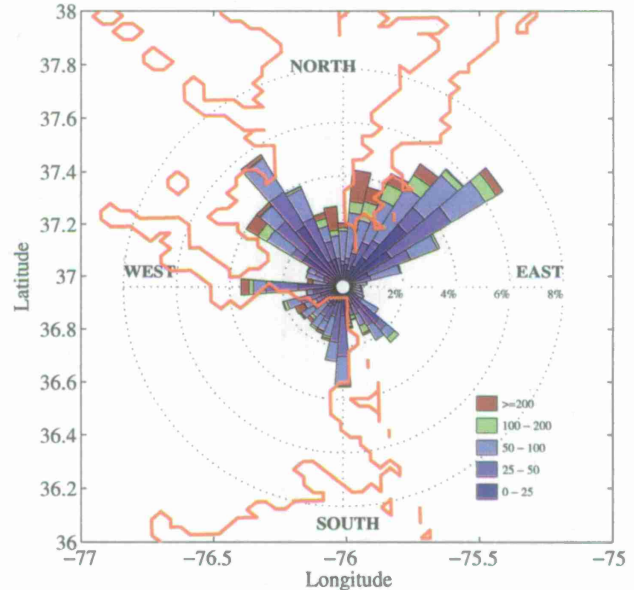
Fig. 26 A wind rose located at Cape Henry for 4–14 June 2010 depicting frequency of occurrence (in percent) and magnitude of the current error (color). The shoreline from the 3-km COAMPS is depicted in red
