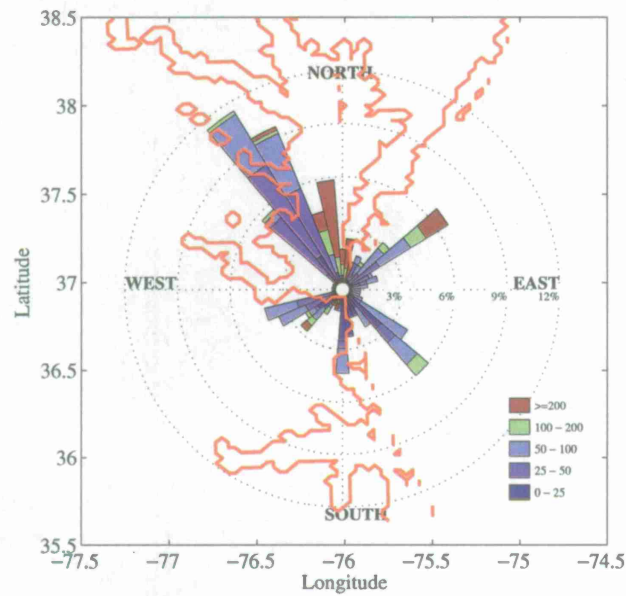
Fig. 23 A wind rose located at Cape Henry for 8–10 June 2010 depicting frequency of occurrence (in percent) and magnitude of the current error (color). The shoreline from the 3-km COAMPS is depicted in red
