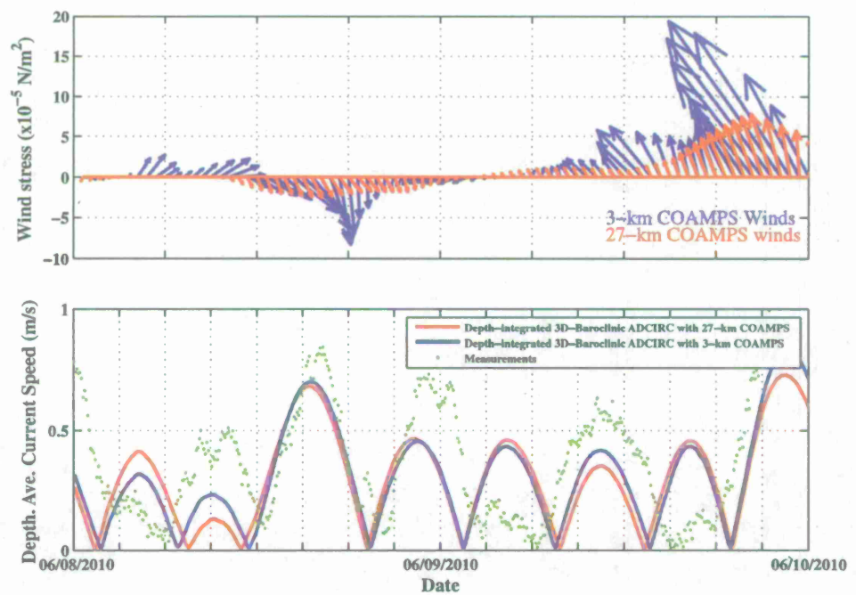
Fig. 17 Two-day model forecasts of baroclinic currents compared to observed currents (green) (both depth-averaged) from 8 to 10 June 2010 together with the applied COAMPS wind magnitude and direction from the 27-km (red) and 3-km (blue) resolution products
