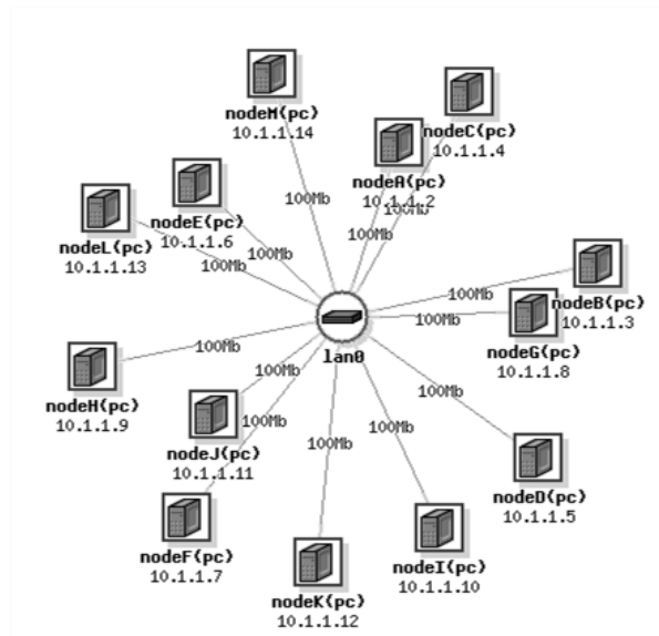
Figure 8: WHB with standard Snort rules trial
