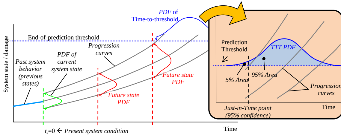
Figure 6. Determination of the prediction time to reach a prognostic threshold with a given prognostic confidence (the inlay box provides an example using 95% confidence)
