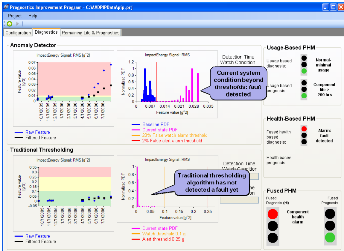
Figure 12. PIP diagnostics results screen (after fault detection)
