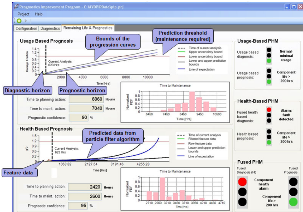
Figure 13. PIP prognostics results screen
