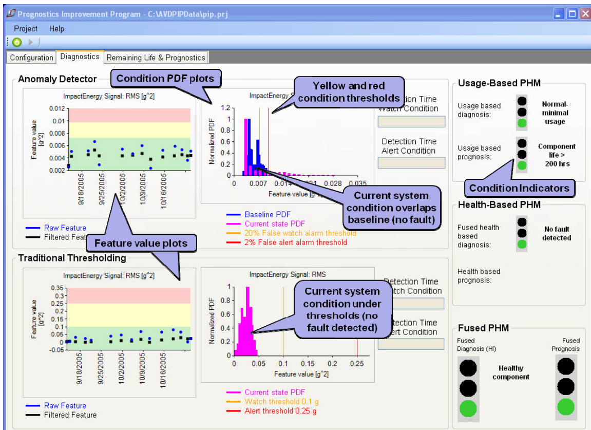
Figure 11. PIP diagnostics results screen (before fault detection)
