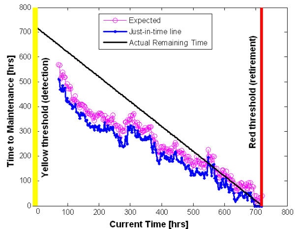
Figure 14. Proposed path to health based prognostics validation
