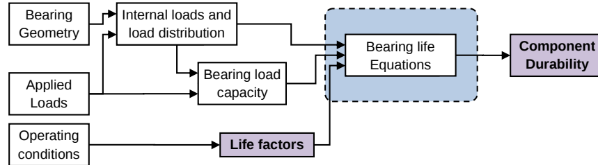
Figure 3. Approach to usage-based bearing lifing used by AVDPIP
