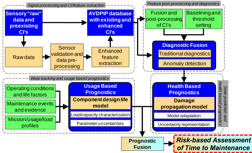
Figure 1: Block diagram of the AVDPIP architecture.
