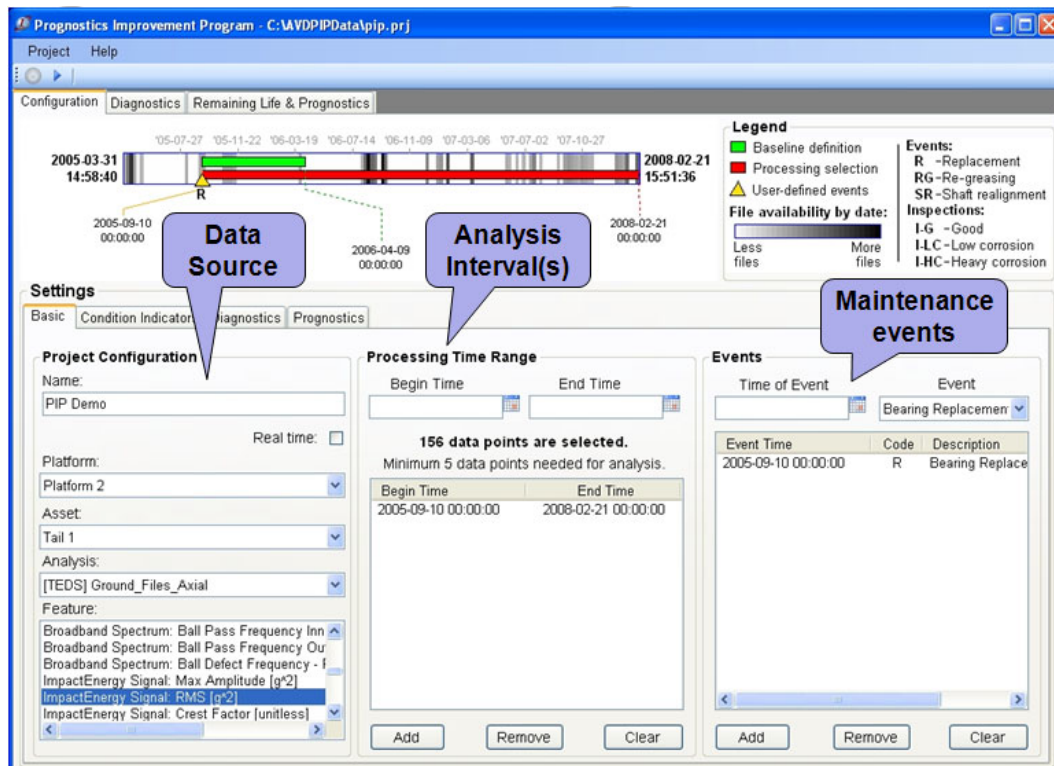
Figure 9. Basic options for setting up an analysis in the PIP tool.
