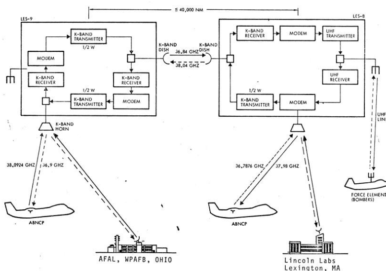
Figure 2 Les-8/9 Satellite System operation
