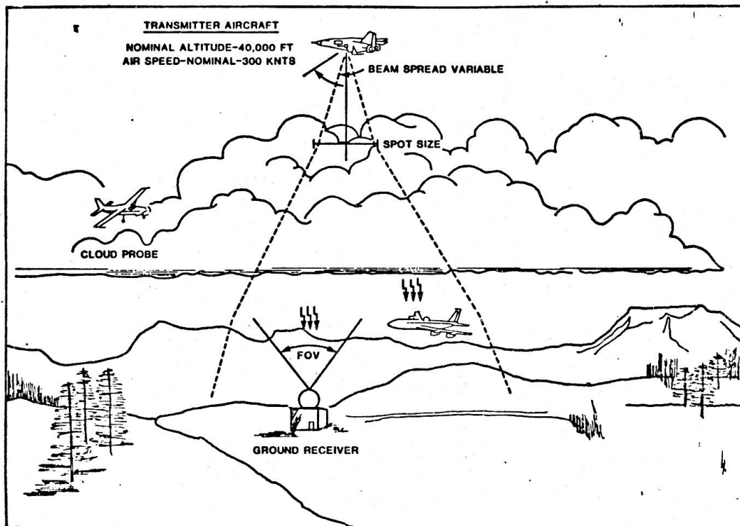
Figure 4 Cloud Experiment Configuration
