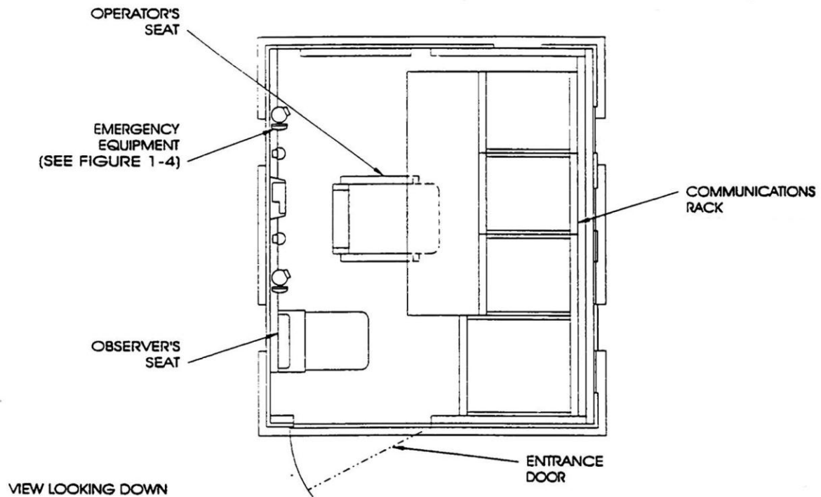
Top View of Communications Module
