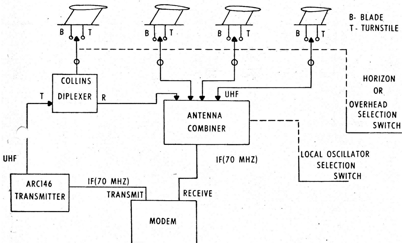
Figure 6 Block Diagram of Proposed Antenna System
