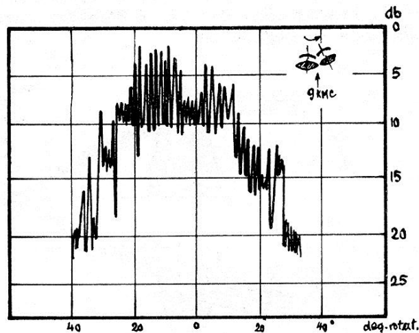
Figure 5 Reflection Pattern of a Lens-Reflector Pair
