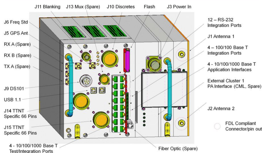
Figure 1 TTNT Phase III Hardware Drawing
