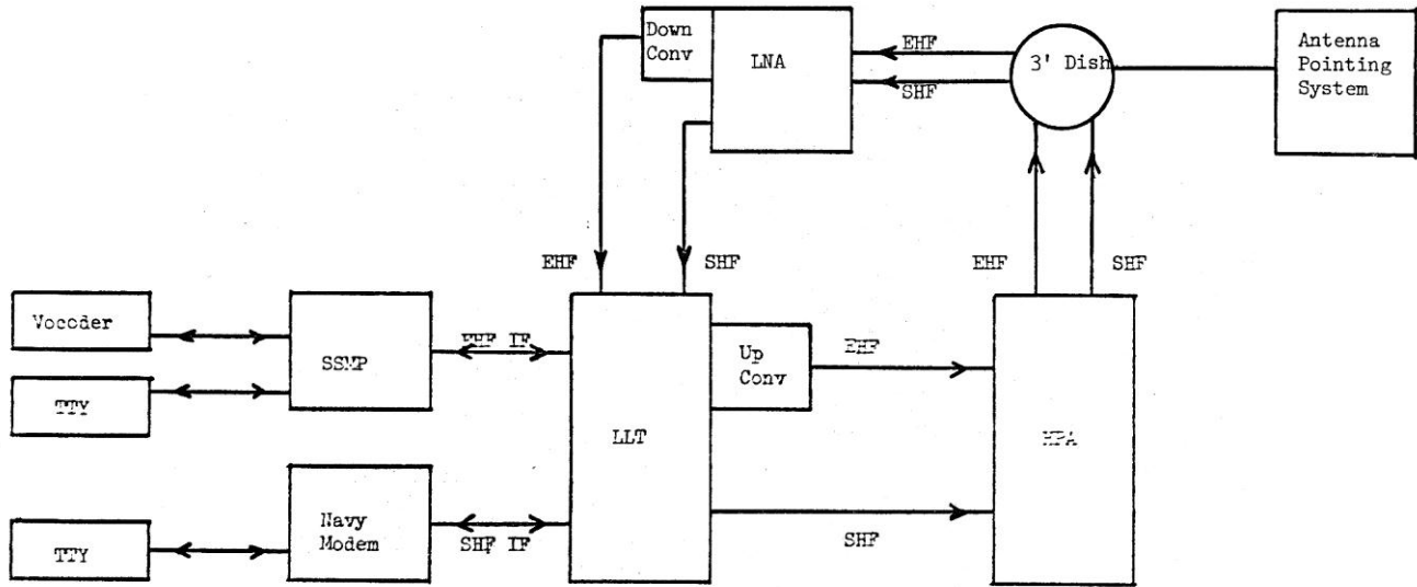
Figure 5 AN/ASC-28 Dual Frequency SATCOM System
