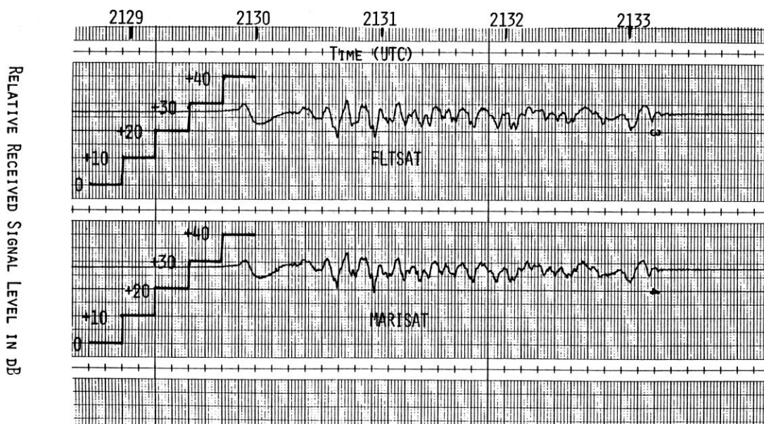
Figure 5 Received Satellite Signal Fading Caused by Ionospheric Irregularities
