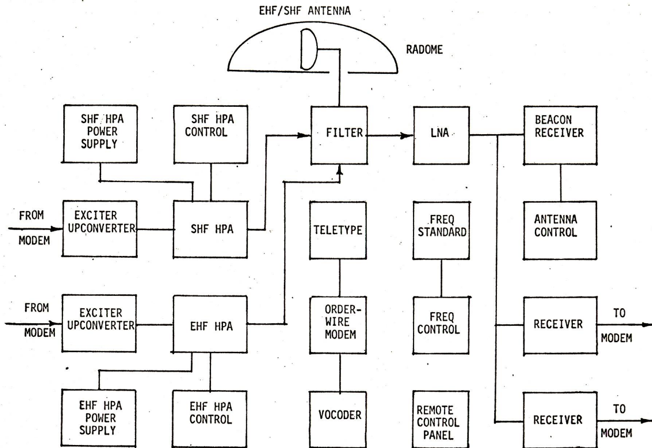
Figure 11 AN-ASC-30 Block Diagram
