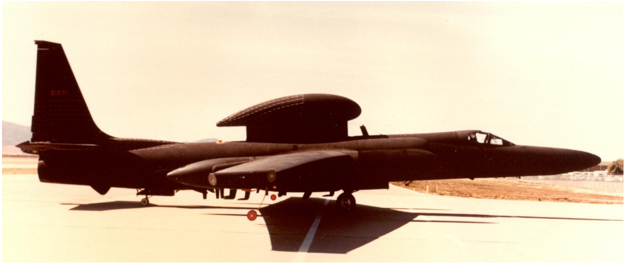
TR-1 with Senior Span Data Link
