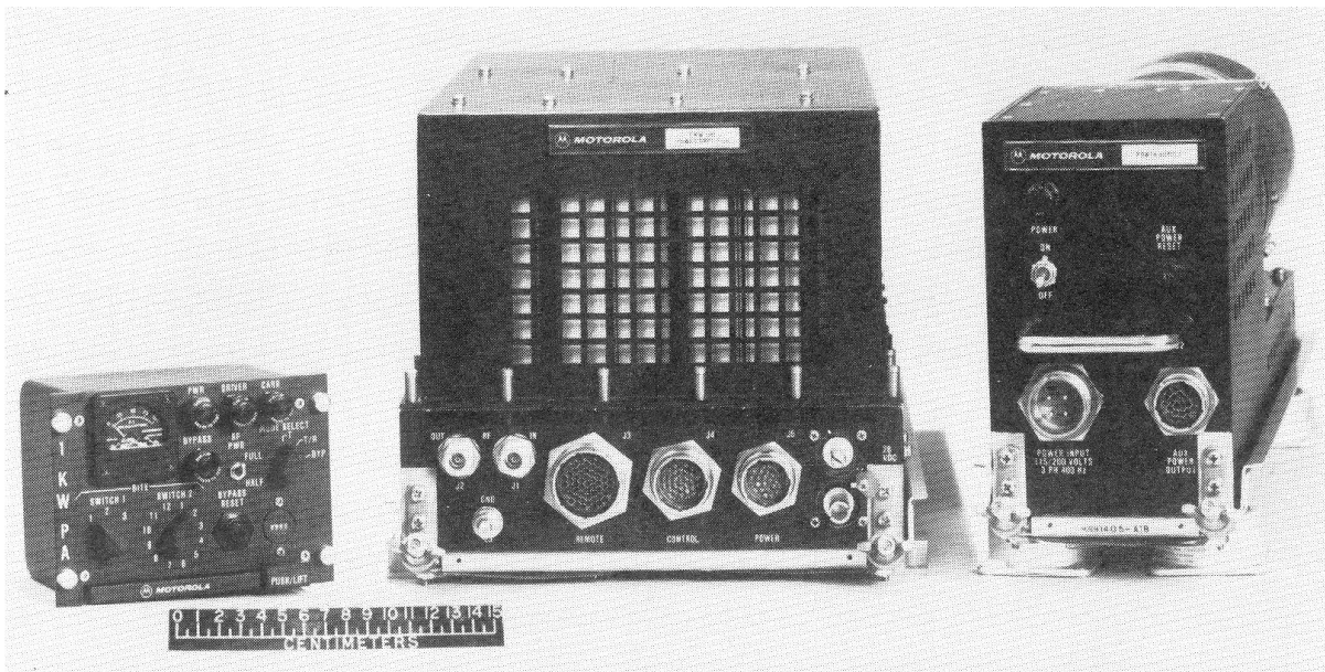
Figure 1 One Kilowatt UHF Solid State Power Amplifier (AN/ASC-31)
