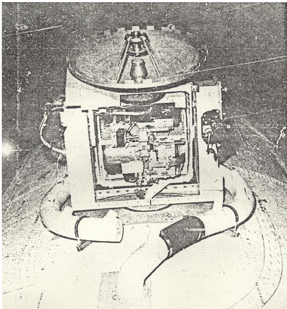
Two-foot X-band antenna on C-121 with Maser Amplifier and Liquid Helium Cooling
