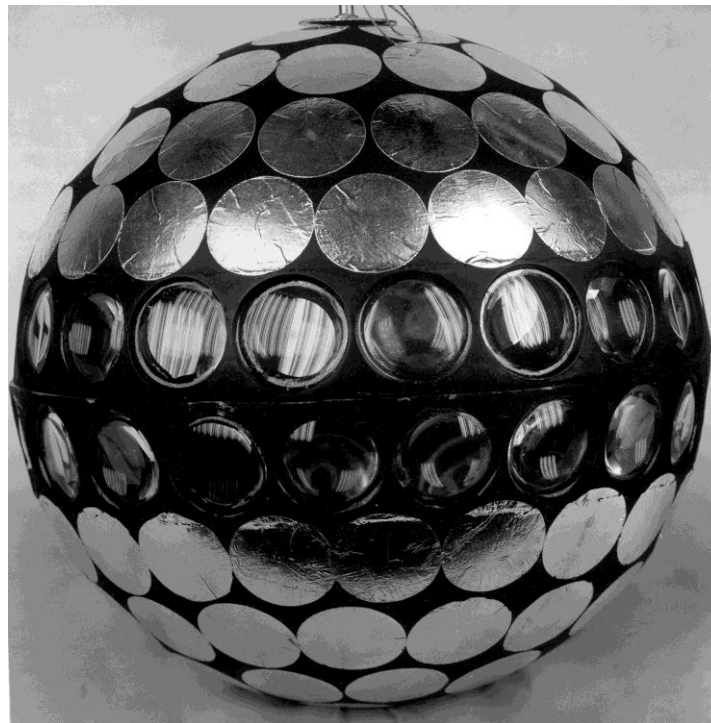
Figure 3 Optical Model of Focused Reflector Sphere
