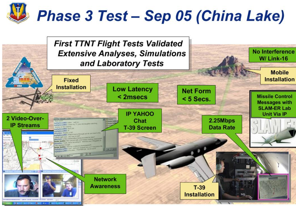
Figure 3 TTNT Phase III Flight Test
