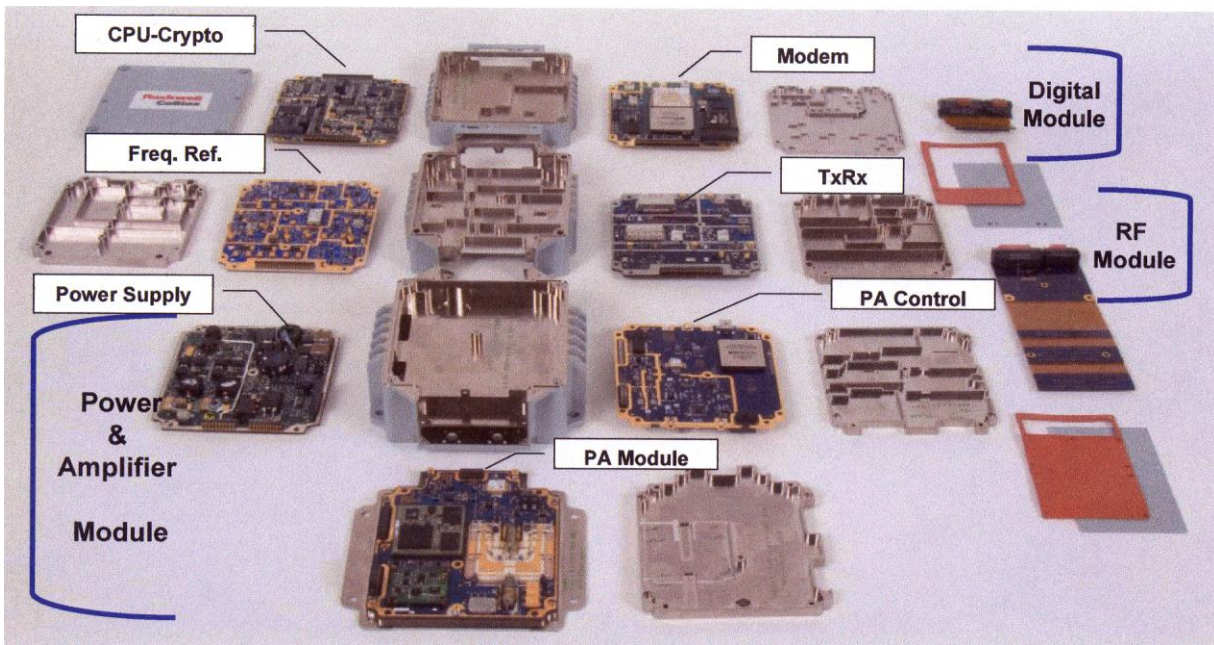
Exploded View of WDL Hardware
