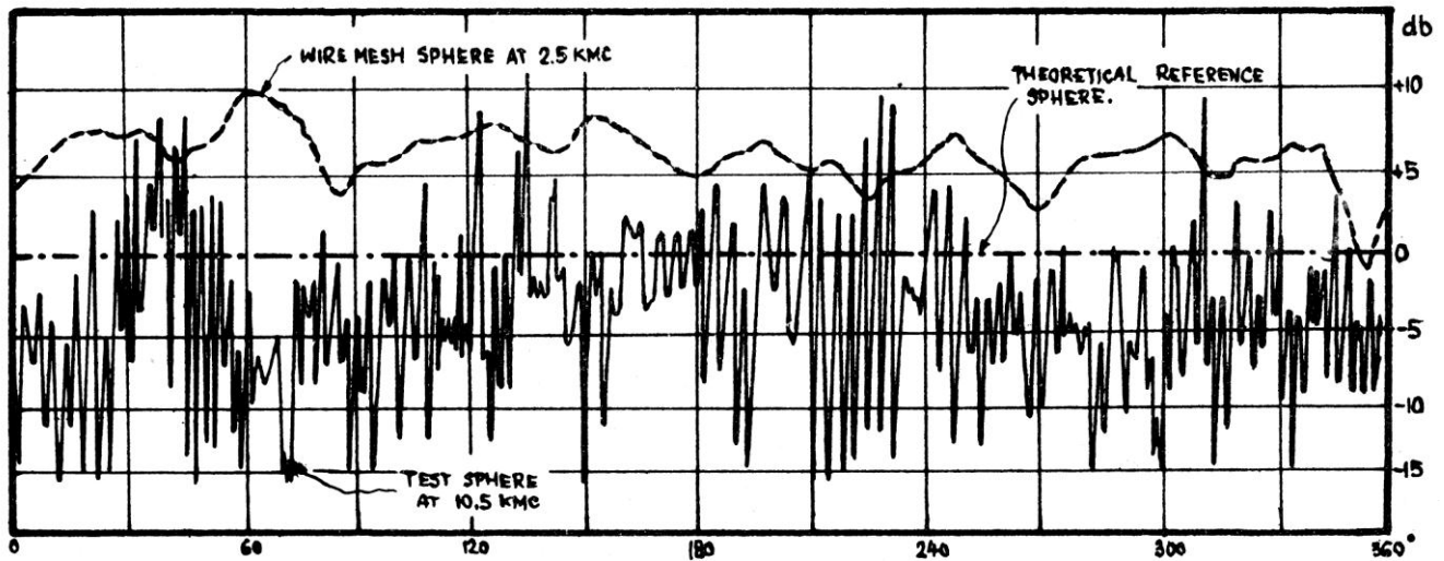
Figure 3 Reflection Patterns of Wire Grid Sphere
