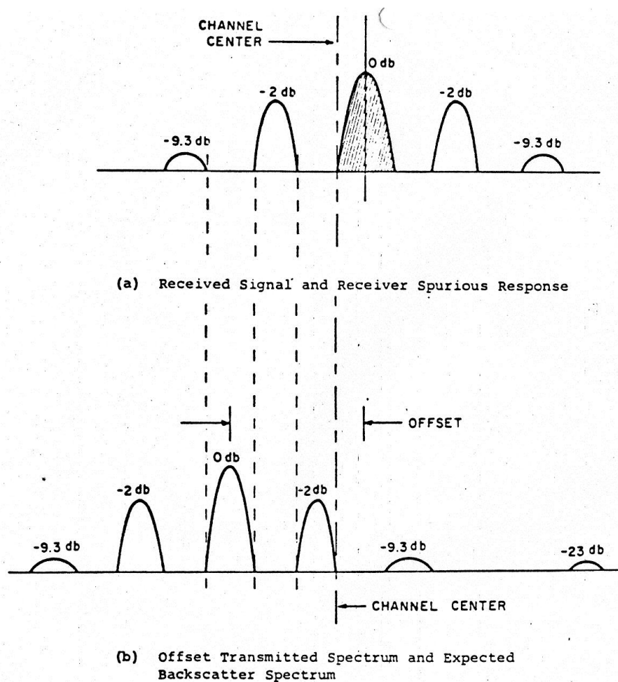
Figure 3 In-Channel Offset
