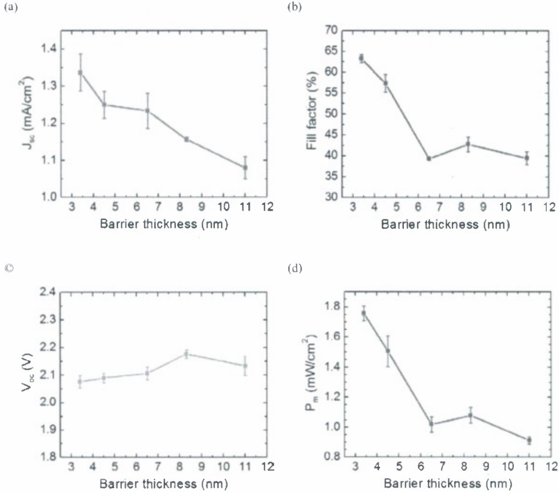
Fig. 14.3. (a) Dependence of J_{sc} on barrier thickness for the series of (20-21) solar cells with varying barrier thickness. (b) Dependence of FF on barrier thickness for the same set of devices. (c) Dependence of V_{oc} on barrier thickness for the same set of devices. (d) Dependence of P_m on barrier thickness for the same set of devices.
