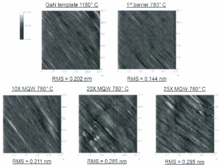
Fig. 12.3. (a) 12.5\ \mu\text{m} \times 12.5\ \mu\text{m} AFM images and measured RMS roughness values for a (20\bar{2}1) GaN template grown at 1180\ ^\circ\text{C} , a (20\bar{2}1) GaN template grown at 1180\ ^\circ\text{C} followed by an 8 nm barrier at 780\ ^\circ\text{C} , and a set of (20\bar{2}1) MQW structures with a varying number of QWs.
