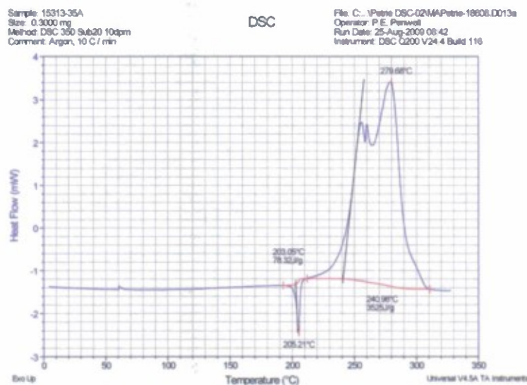
Figure 2. DSC of 1,1'-diamino-4,4',5,5'-tetranitro-2,2'-biimidazole, 3 .
