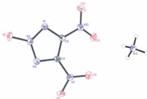
Figure 6. ORTEP drawing of ammonium 2-oxy-4,5-dinitro-1,2,3-triazole (AODNTz), 16 .
