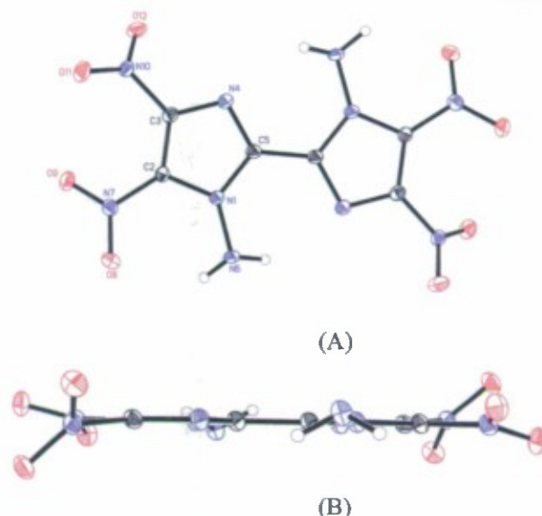
Figure 1. Overhead (A) and side (B) ORTEP views of 1,1'-diamino-4,4',5,5'-tetranitro-2,2'-biimidazole, 3 .
