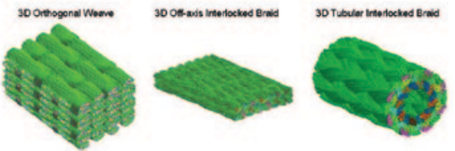
Figure 1: 3-D Fabric Fiber Architectures Generated by Using the Textile Process Simulation Code.
