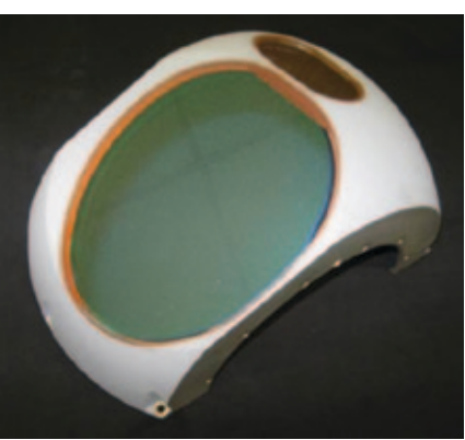
Hot-pressed spinel window for Advanced Targeting - Forward Looking Infrared targeting pod (AT-FLIR).
