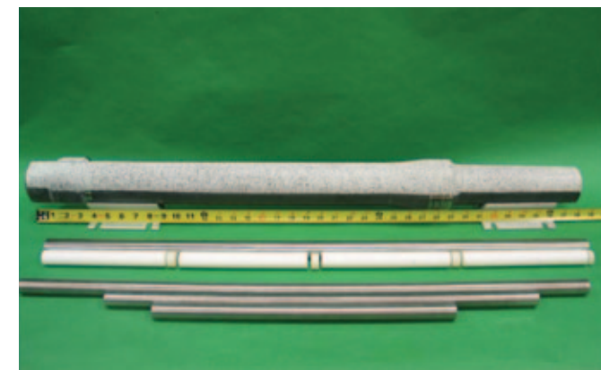
GLEEM Hardware: In the background is the truncated M242 gun tube (the speckle pattern applied is for optical strain measurements). The steel rods in the foreground are used to apply pressure to the elastomeric material and seals (white rods) as they are inserted one at a time into the liner.
