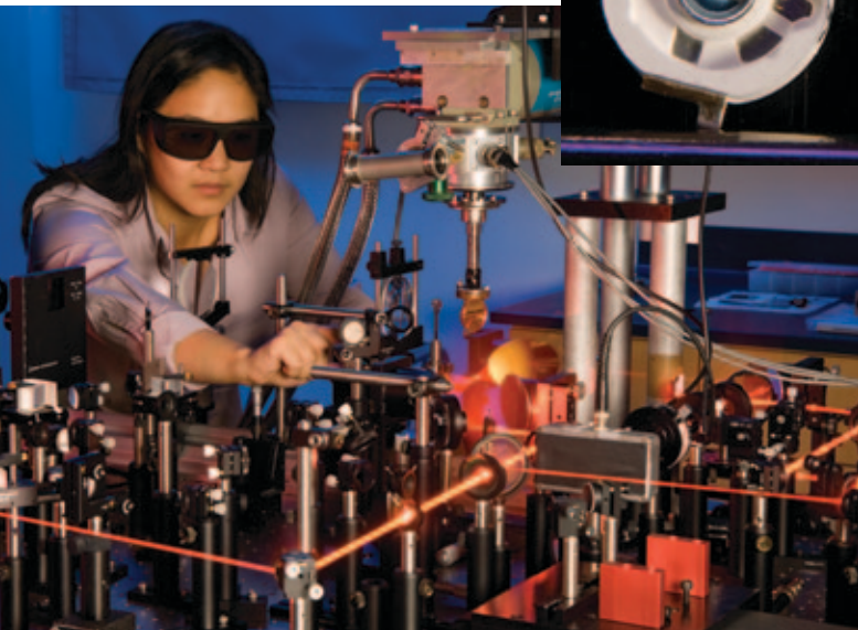
Dr. Grace Metcalfe performing UV pump and terahertz probe spectroscopy measurements to study carrier dynamics in ARL-grown nanometer-scale compositional inhomogeneous AlGa N materials. Inset photo: Electroluminescence from a deep ultraviolet light emitting diode packaged on a surface mount header.
