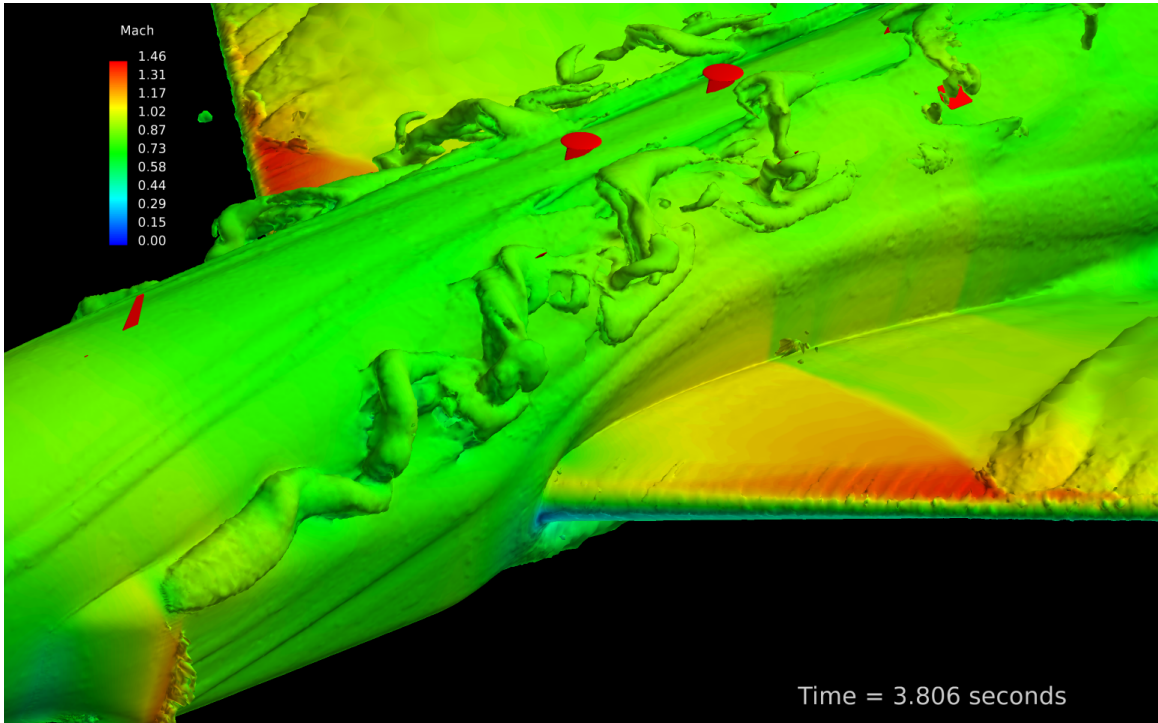
Figure 4.23: Rivet Joint with LCS ( AoA = 8^\circ ) – vorticity of 100 Hz colored by Mach number for high angle of attack study (antennas colored by red shown for reference locations only – not included in solution)
