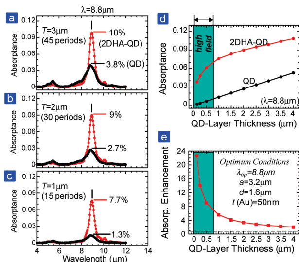
FIGURE 6. Optimum conditions for plasmonic-QD interaction. (a-c) The calculated absorbance spectra of a 2DHA-QD sample (the red curves) with three different QD layer thicknesses, T = 3 , 2 , and 1 \mu\text{m} , respectively. The spectra for the QD samples, shown as the black curves, are for reference. The enhanced QD absorption occurs at \lambda \sim 9 \mu\text{m} , i.e., the plasmonic- \lambda of the 2DHA structure. (d) A summary plot of peak absorbance as a function of T for the 2DHA-QD (the red circles) and the QD (the black circles) samples. The green color indicates the region where a strong plasmonic-field exists. (e) A plot of absorption enhancement as a function of T for an optimum 2DHA-QD sample ( a = 3.2 \mu\text{m} , d = 1.6 \mu\text{m} , and t = 50 nm). The data show that an enhancement of as much as 10 times can be achieved at T = 0.5 \mu\text{m} .
