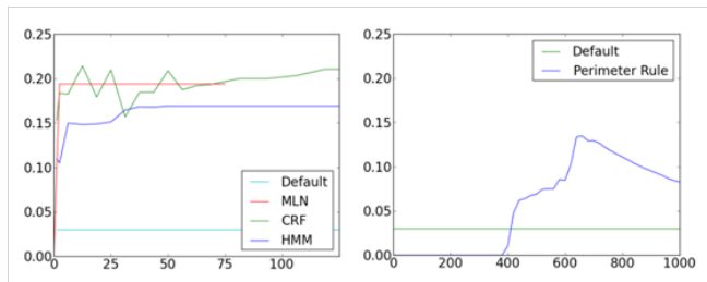
Figure 2: F_1 scores during training while varying (left) PGM window size and (right) Rule perimeter distance threshold.
