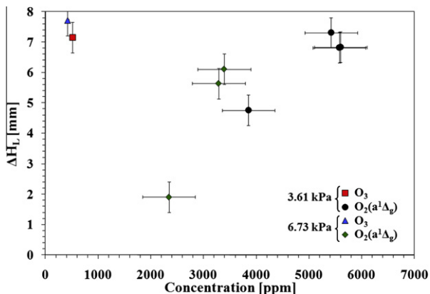
Fig. 11. Plot of experimental results of flame liftoff change with O_2(a^1\Delta_g) and O_3 concentration for a plasma power of 80 W. The error bars denote the experimental uncertainties in the concentrations and change in flame liftoff height.
