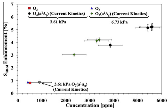
Fig. 12. Plot of computational results of lifted flame speed enhancement with O_2(a^1\Delta_g) and O_3 . The horizontal error bars denote the propagation of uncertainty from the concentrations found experimentally, while the vertical error bars denote the range of lifted flame speed enhancement when using the different published reaction rates.
