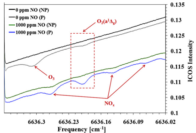
Fig. 4. ICOS transmittance spectrum with and without NO addition and plasma activation (P and NP are plasma and no plasma, respectively).
