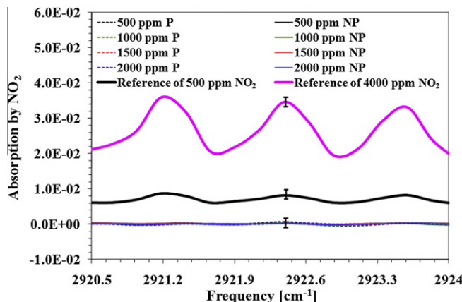
Fig. 9. NO_2 absorption measurements from FTIR showing that the NO is not converted to NO_2 when the plasma is on or off (P and NP are plasma and no plasma, respectively).
