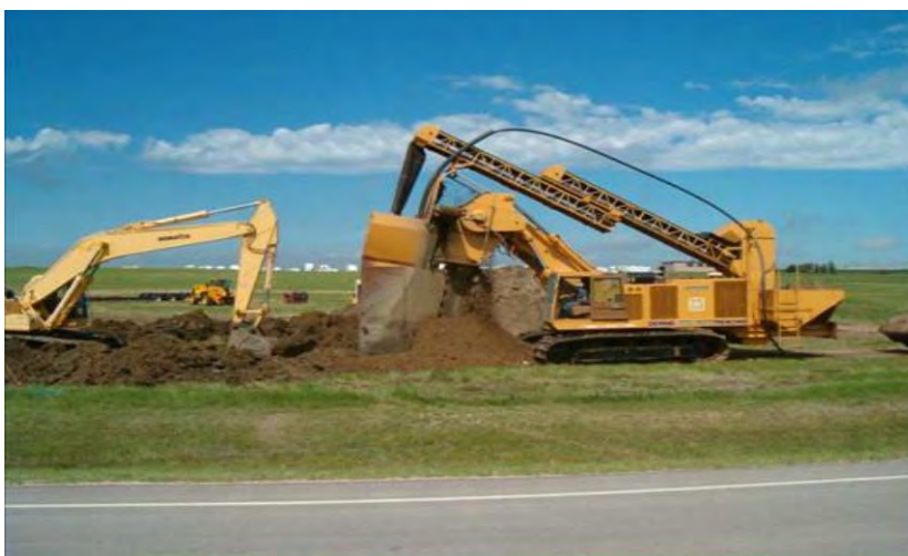
Figure 6-3. Continuous chain trencher at Ellsworth AFB, South Dakota. (Courtesy of the U.S. Air Force)
