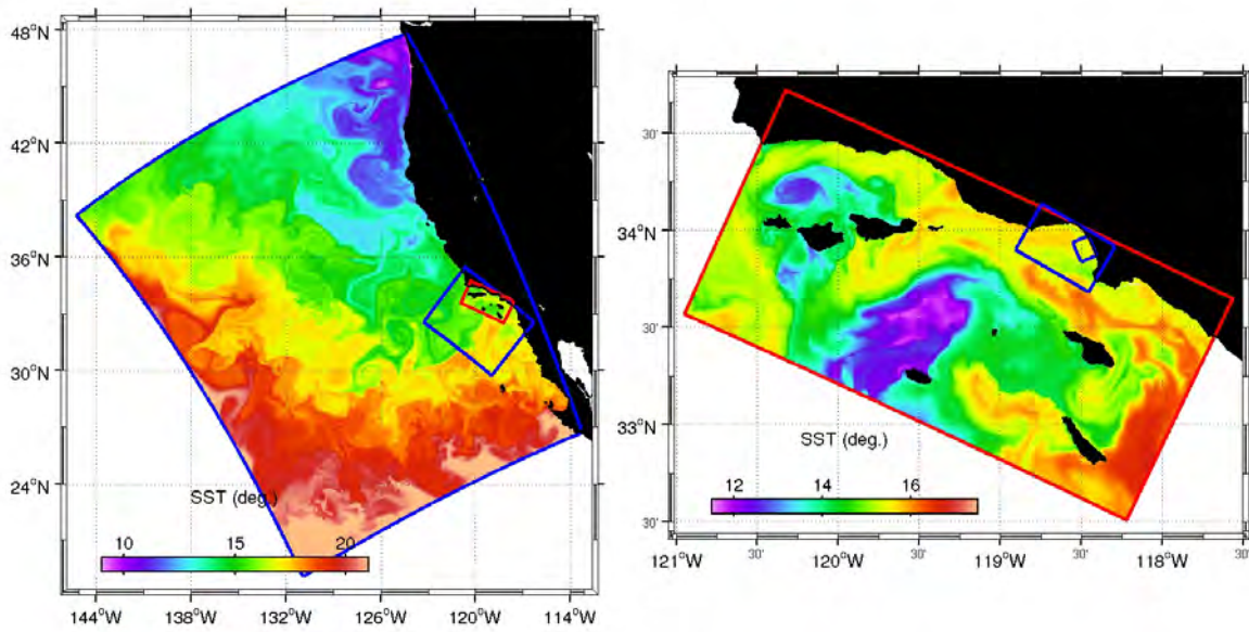
Figure 4: Snapshot of SST in successive grid nests starting at the scale of the Eastern Subtropical Pacific ( dx = 4 km) descending down, in this application, to the Santa Monica Bay ( \Delta x = 20 m). It is used to simulate local phenomena of mesoscale and submesoscale eddies, internal tides, and nearshore surface wave breaking and rip currents (Uchiyama et al., 2010). The methodology is most recently explained in Mason et al. (2010).
