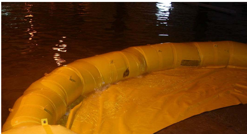
Figure 3.2. Successful small-scale test of a single-arch system for blocking flow across a large open area. The actual distance spanned by the ARCH in this test is about 25 ft.
