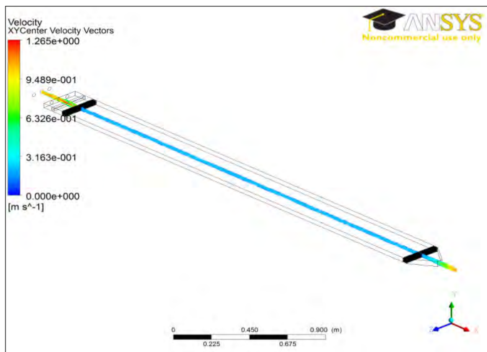
Figure 21. Velocity Vectors at XY Plane at Center of Duct with Honeycomb Structures
