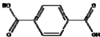
Figure 2. Chemical Structure of a Multifunctional Acid [Terephthalic Acid]
