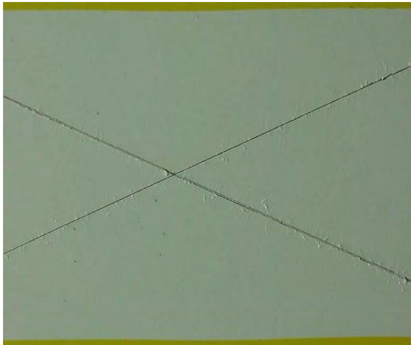
Figure 27. LTCPC Filiform Corrosion Resistance Test Outcome – Retest
