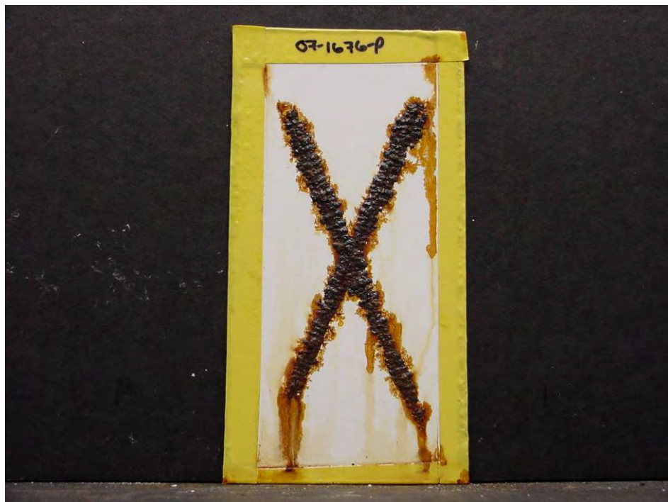
Figure 26. Control Coating Cyclic Corrosion Resistance Test Outcome – Steel
