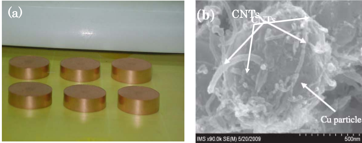
Figure 11. (a) optical image (b) surface morphology of Cu/CNTs nanocomposites with 1wt% of CNTs
