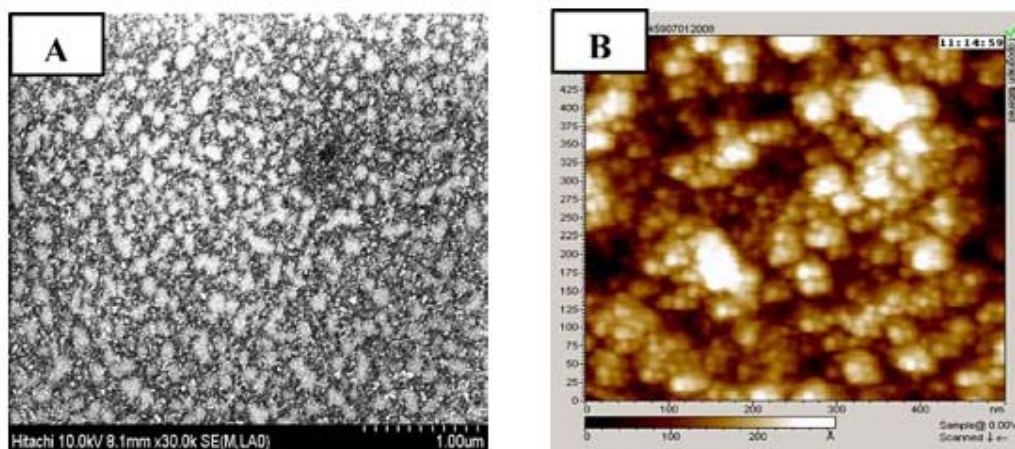
Figure 3. (A) SEM and (B) AFM images of the \text{Fe}_3\text{O}_4 nanoparticles on the \text{Si}/\text{SiO}_2 surface (see online version for colours)
