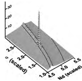
FIG. 17. 3D map of the least-squared solution of Eq. (4) using as input data the hypothetical case illustrated in Fig. 11(b) with D_m = 350 nm, N_d = 5 \times 10^{16} \text{cm}^{-3} , and \sigma_n = 1 \times 10^{-21} \text{cm}^2 . The map is scaled such that N_d ranges from 4.5 \times 10^{16} to 5.5 \times 10^{16} \text{cm}^{-3} and \sigma_n ranges from 5 \times 10^{-22} to 1.48 \times 10^{-21} \text{cm}^2 . The vertical axis is the negative logarithm of the least-squared deviation between the input and computed normalized photoconductive decay and is arbitrarily truncated at a value of 30. The pole conforms to a solution coincident with the values of N_d and \sigma_n used to generate the input data. The locus of minima appearing as a continuous “ridge” traversing diagonally across the map conforms to the solution of the limiting case where \Phi(t) \rightarrow \phi_m .
