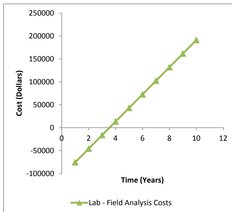
Figure 7.2. Difference in cost between the traditional laboratory analysis and the field analysis. Break-even point occurs at 3.54 years.
