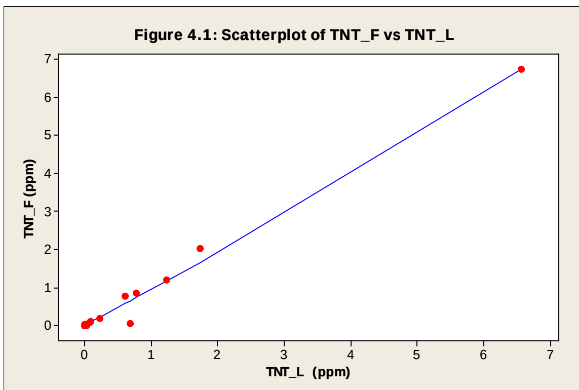
Figure B10. Scatter plot of all detected results for TNT.
