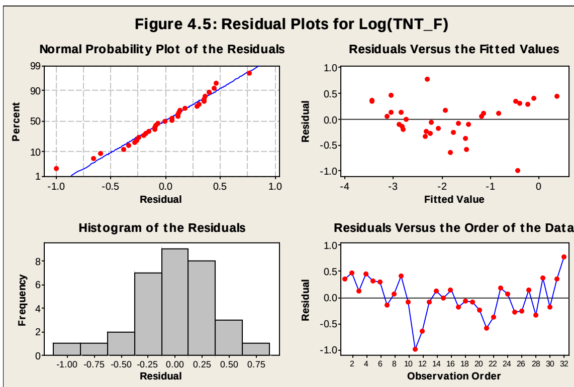
Figure B14. Residual plots for TNT showing relatively poor fit.
