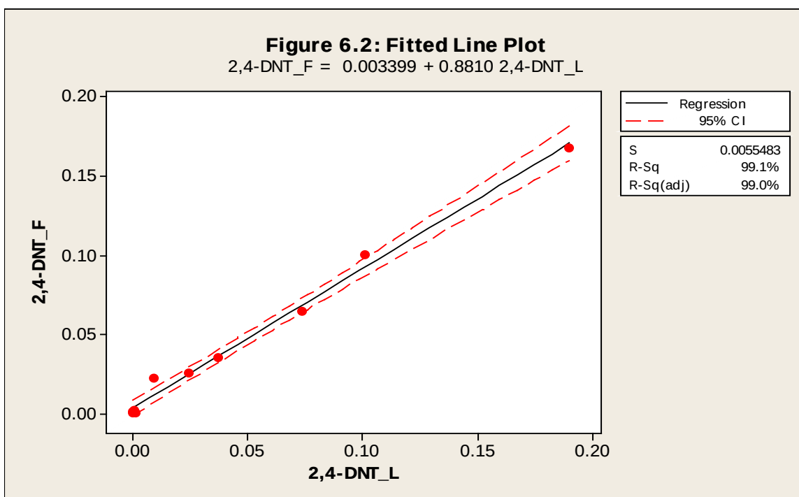
Figure B34. Fitted line plot for 2,4-DNT.
