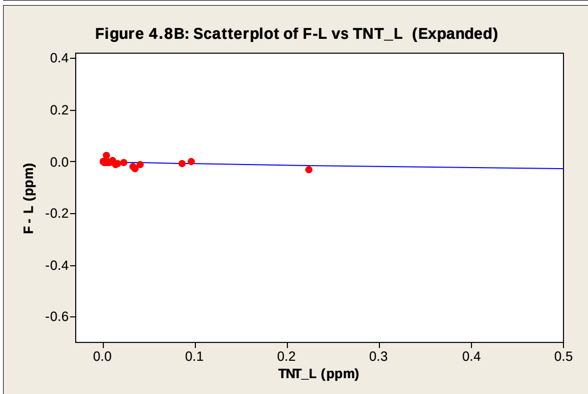
Figure B17. Scatter plots for F-L versus L.
