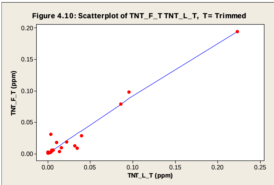
Figure B19. Scatter plot of “trimmed” TNT pair data set.
