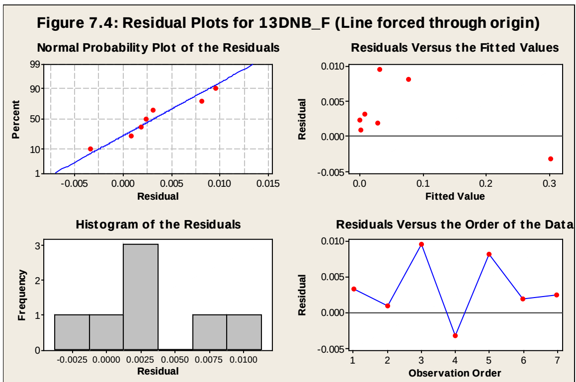
Figure B41. Residual plots for 1,3 DNB, line forced through origin.
