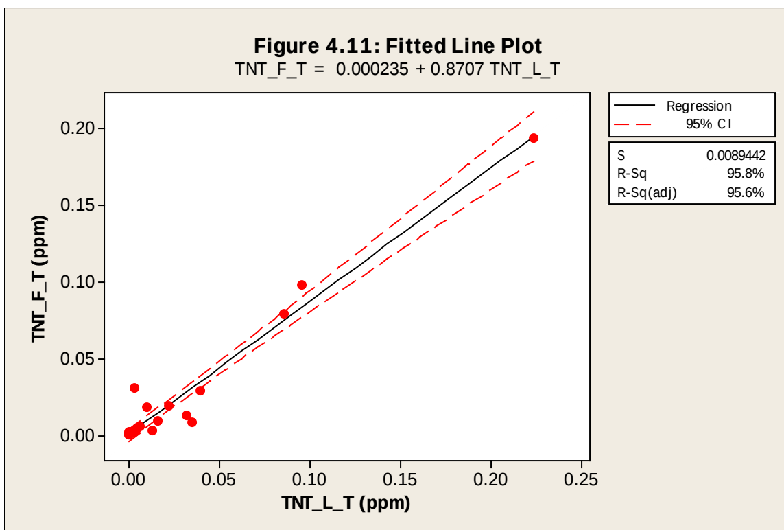
Figure B20. Regression line for trimmed data set.
