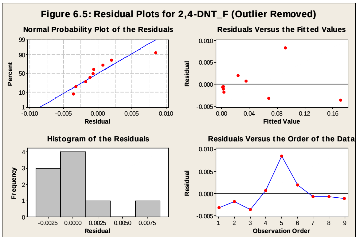
Figure B37. Residual plots for 2,4-DNT, outlier removed.
