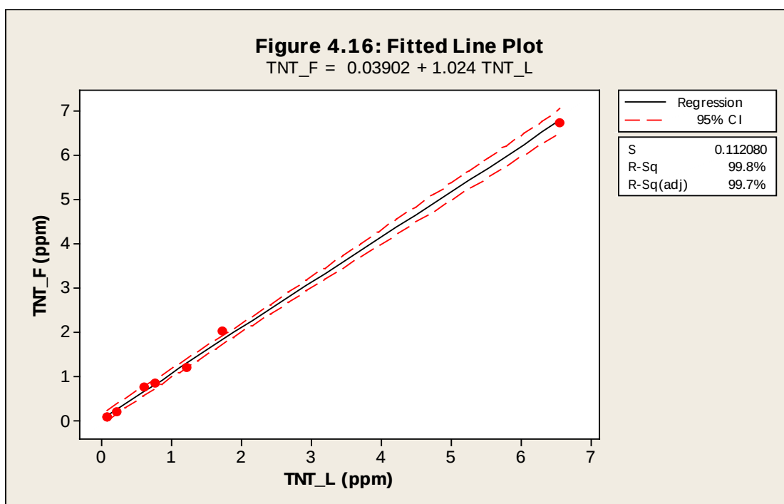
Figure B26. Regression line for “high-level” paired TNT data set.
