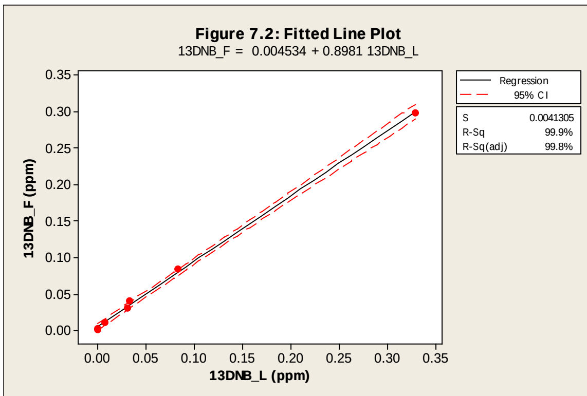
Figure B39. Fitted line plot for 1,3-DNB.
