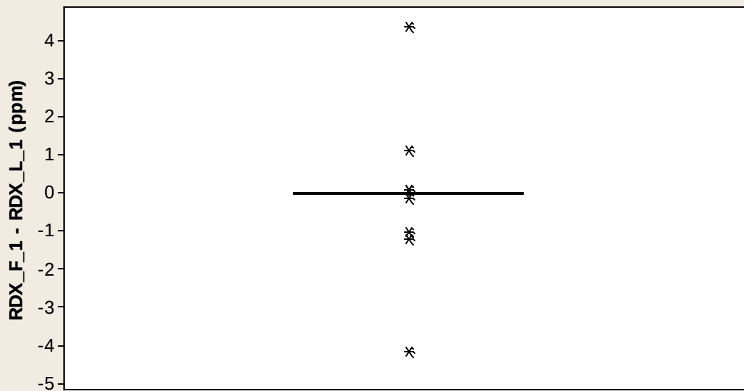
Boxplot of paired differences
