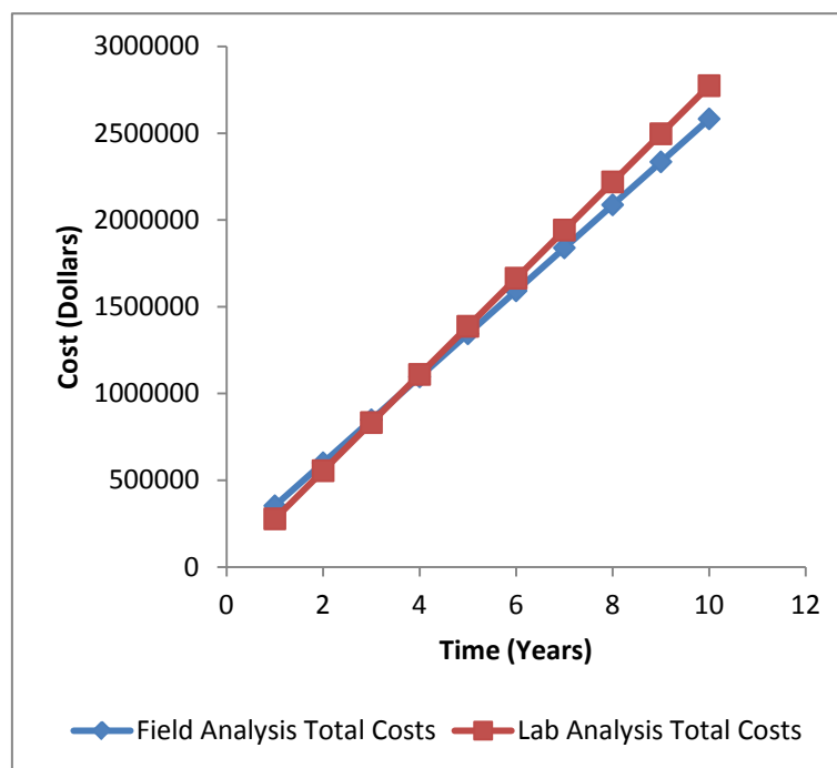
Figure 7.1. Total cost for traditional laboratory ($277,360/year) and field analysis $247,739/year).
