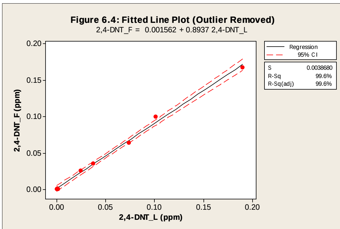
Figure B36. Regression fit for 2,4-DNT, outlier removed.
