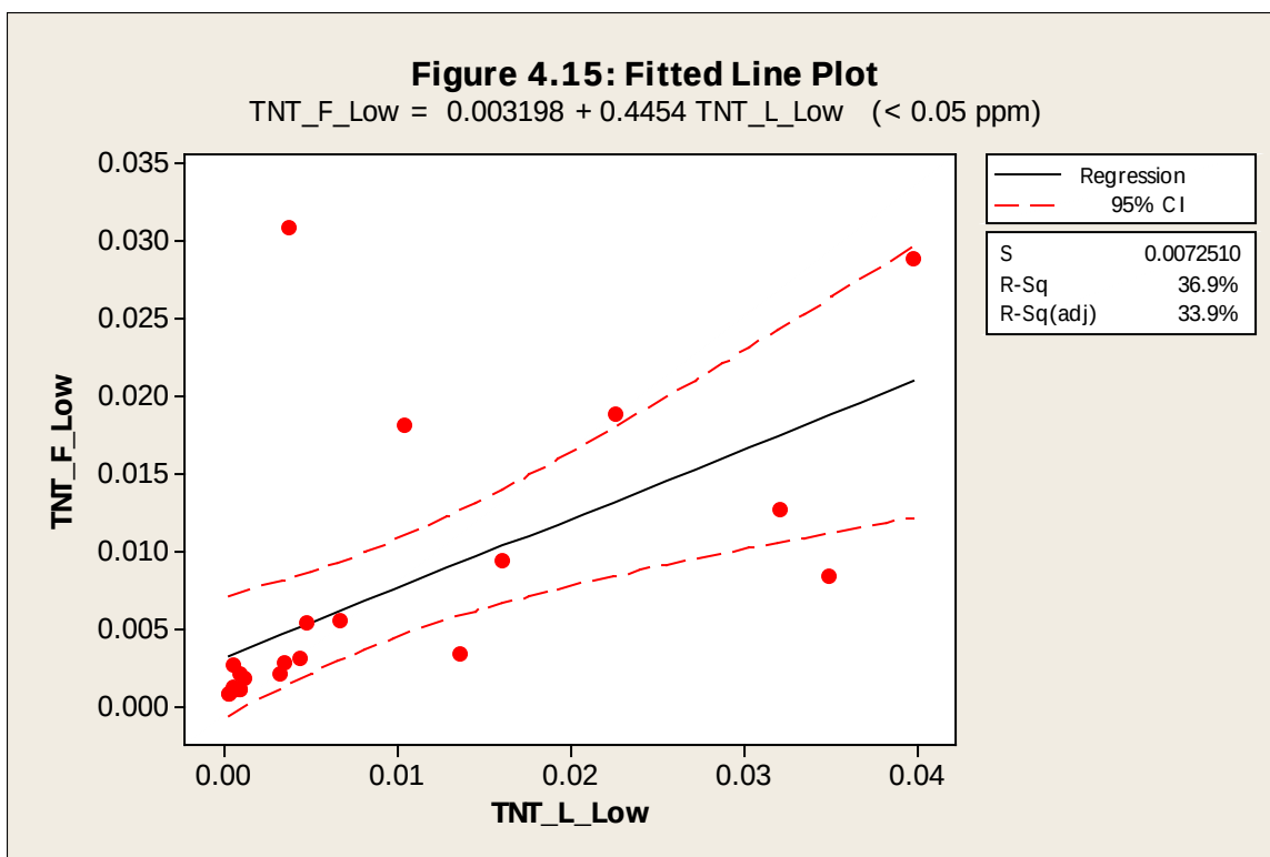
Figure B24. Linear regression fit for detected TNT concentration &lt;0.05 mg/L.
