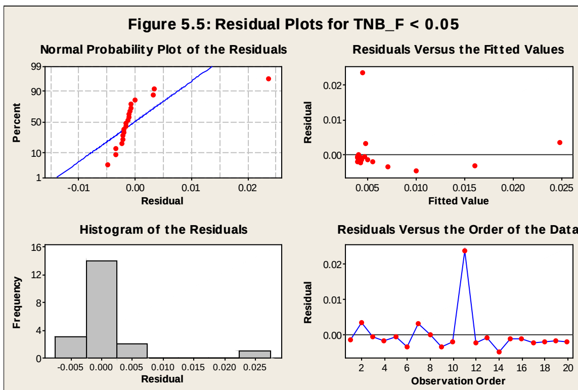
Figure B32. Residual plots for TNB low concentrations.
