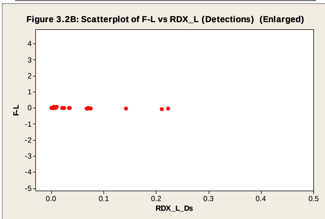
Figure B2. RDX scatter plots showing outlier.
