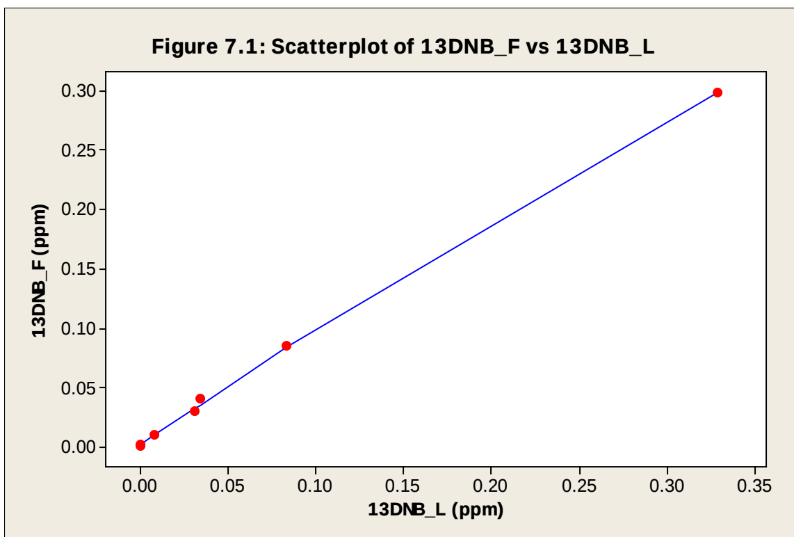
Figure B38. Scatter plot of detected 1,3-DNB results.
