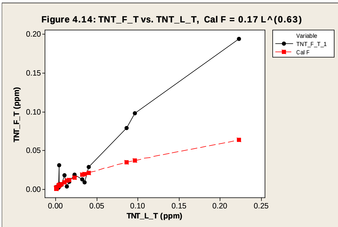
Figure B23. Observed and calculated values of field concentrations for TNT.
