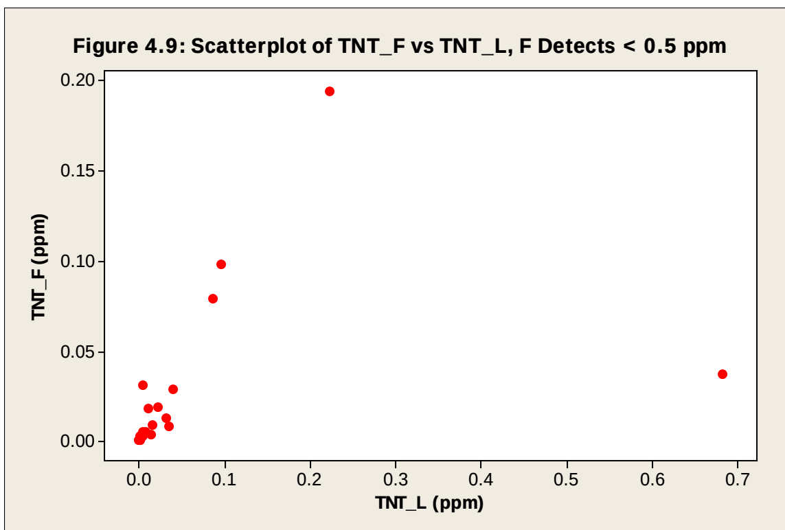
Figure B18. TNT scatter plot showing outlier.
