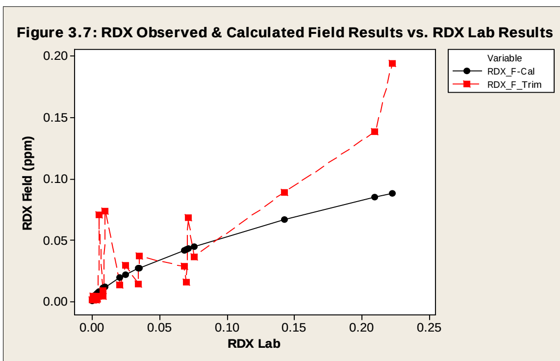
Figure B7. Field results versus lab results for RDX.
