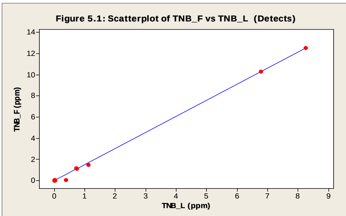
Figure B28. Scatter plot of TNB data set.
