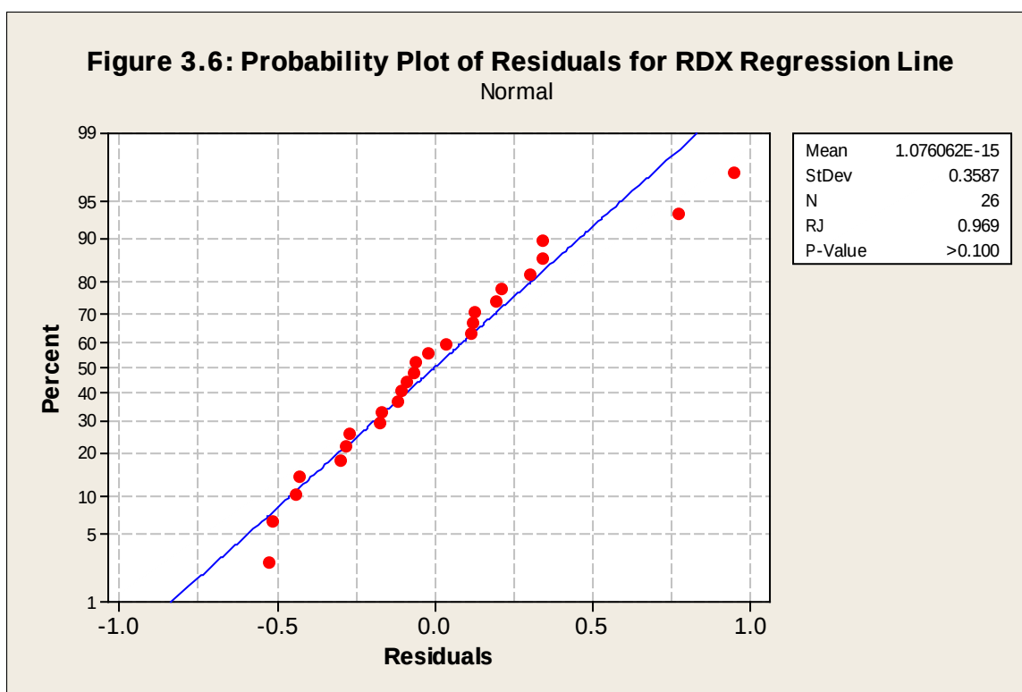
Figure B6. Probability plot of residuals for RDX regression line.
