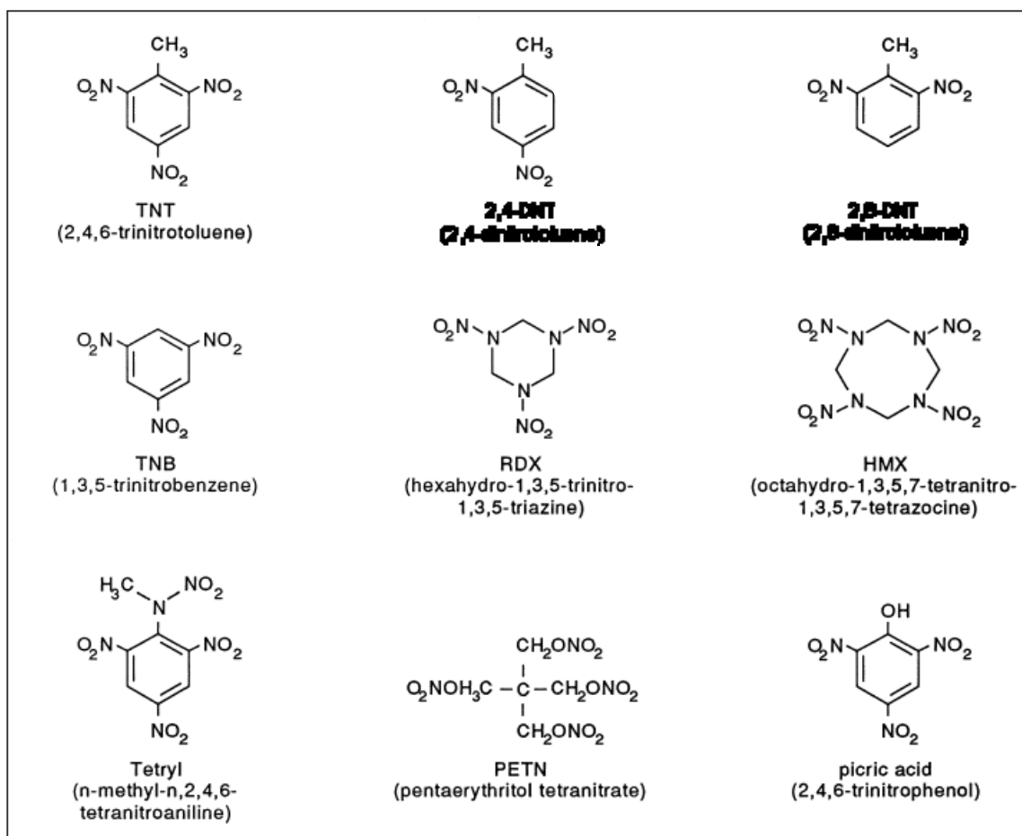
Figure 2.3. Structural representation of known MC present at LAAP.
