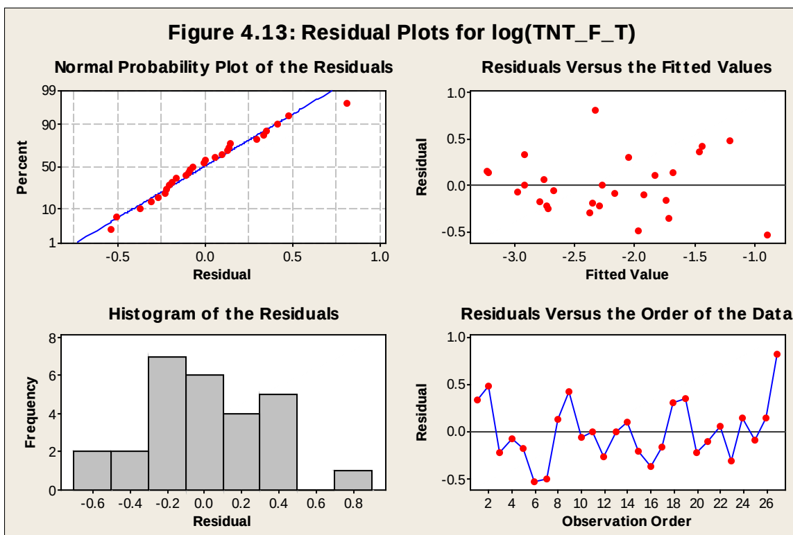
Figure B22. Log normal residual plots for TNT.
