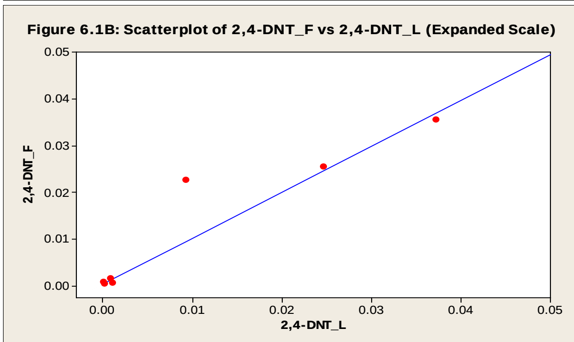
Figure B33. Scatter plots for detected 2,4-DNT results.
