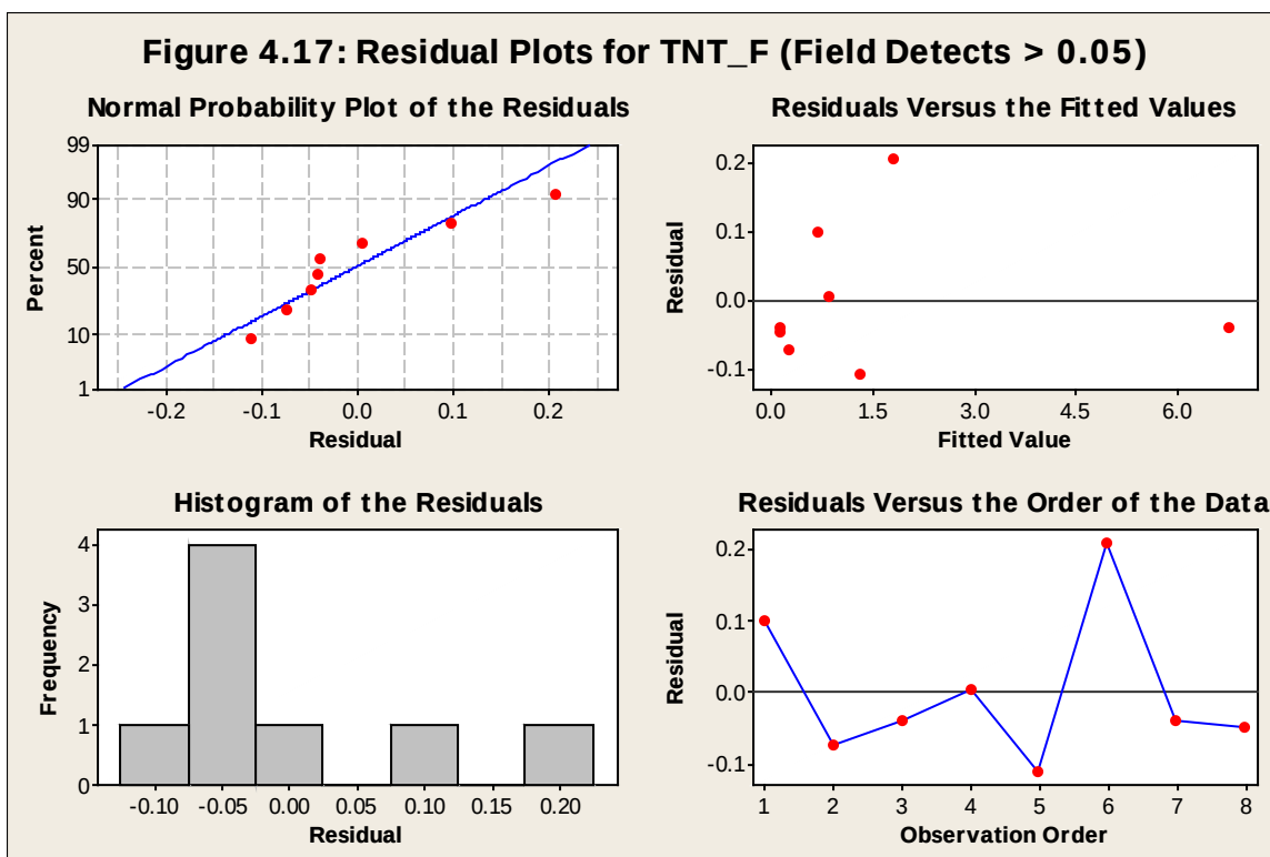
Figure B27. Residual plots for TNT field detects >0.05.
