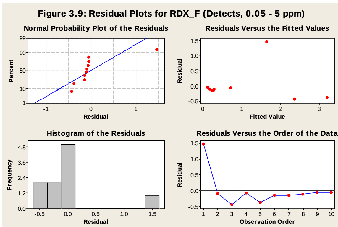
Figure B9. Residual plots for RDX.
