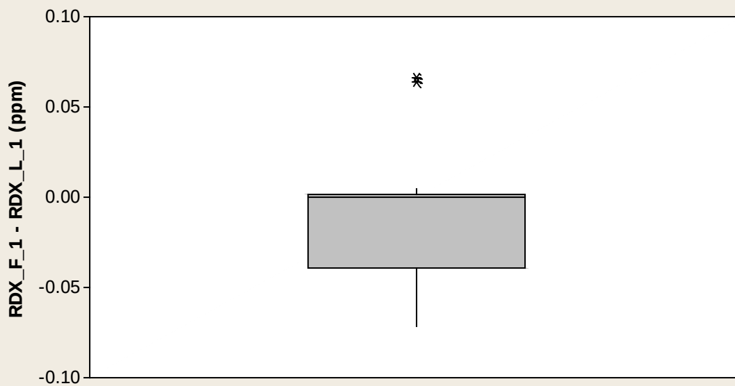
Boxplot of paired differences (Enlarged Scale)
