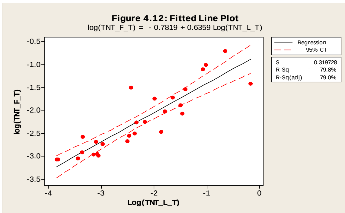
Figure B21. Fitted line plot for TNT.
