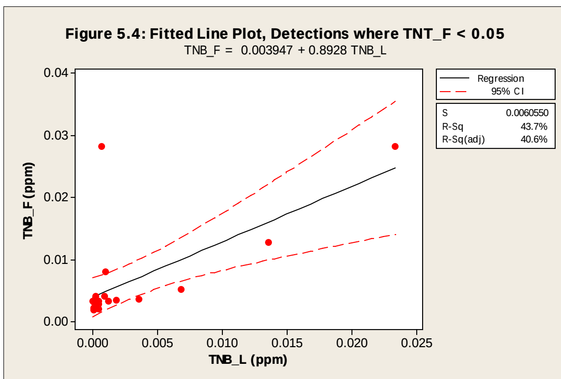
Figure B31. Fitted line plot for TNB low concentrations.
