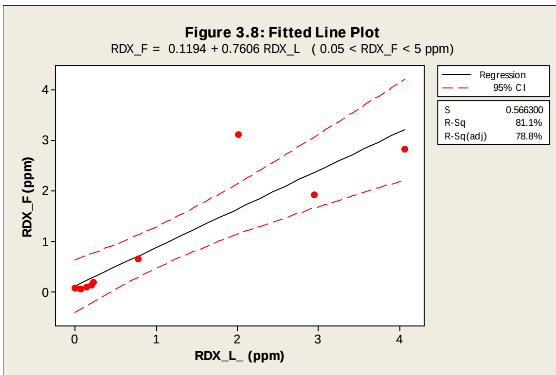
Figure B8. Scatter plot and regression line for RDX.
