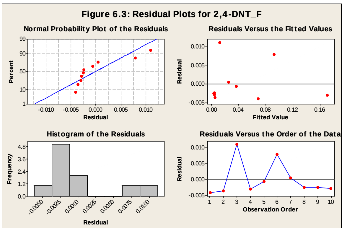
Figure B35. Residual plots for 2,4-DNT.
