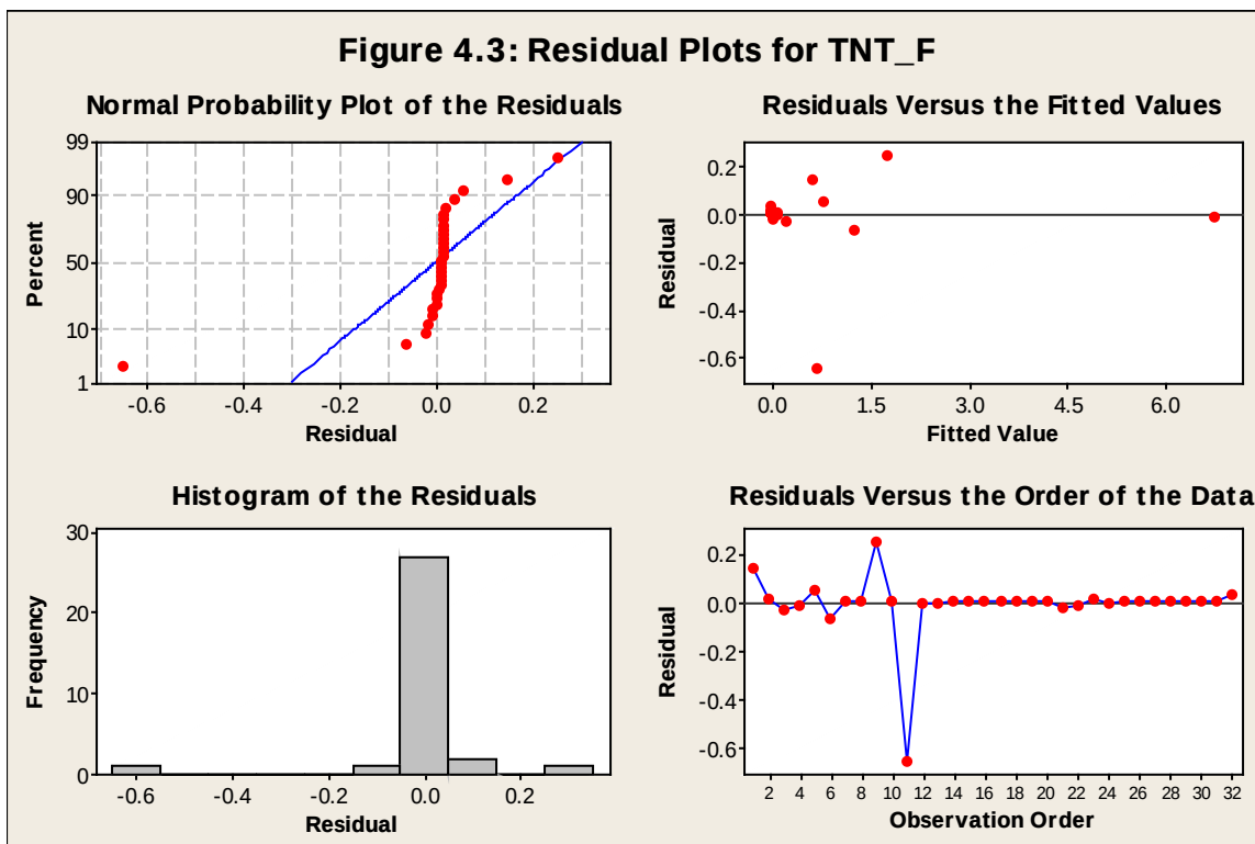
Figure B12. TNT residual plots.
