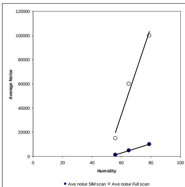
Figure 2.6. Average baseline noise observed on the Griffin 400 for both selected ion monitoring (SIM) and full scan monitoring with varying humidity conditions. Below 55% humidity the average baseline noise is constant.
