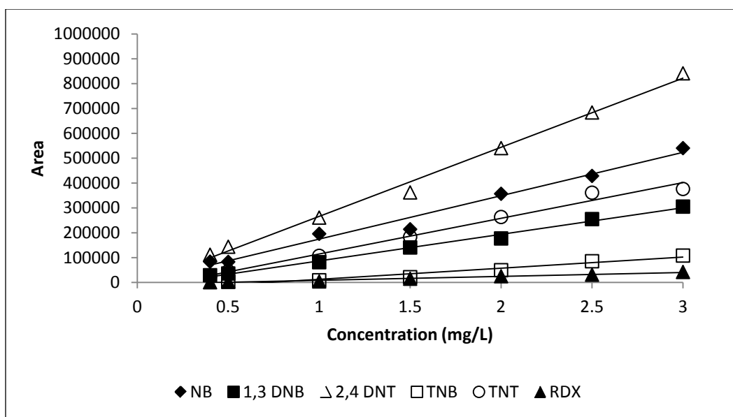
Figure 2.4. Calibration curves for NB, 1,3-DNB, 2,4-DNT, TNB, TNT and RDX.
