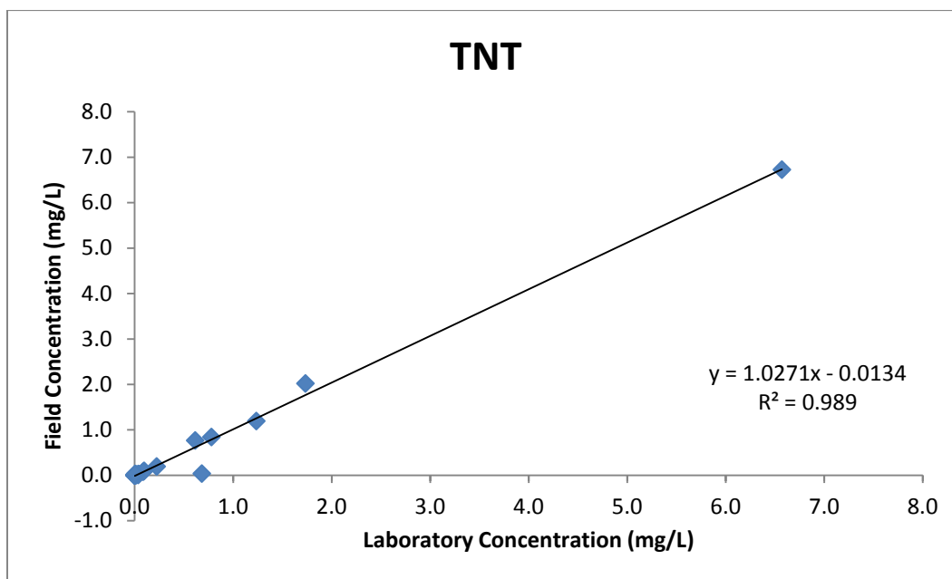
Figure 5.6. Griffin 450 field-analyzed data vs. traditional laboratory analysis by HPLC for TNT.
