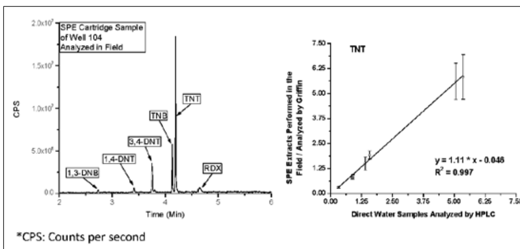
Figure 2.5. Typical chromatogram obtained by the Griffin 400 GC-MS ( left ) and a comparison between the Griffin 400 GC-MS results from the field work and the HPLC Laboratory results for TNT ( right ).
