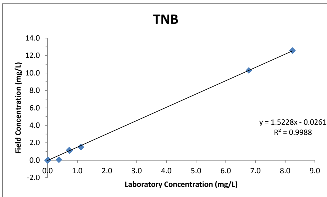
Figure 5.5. Griffin 450 field-analyzed data vs. traditional laboratory analysis by HPLC for TNB.
