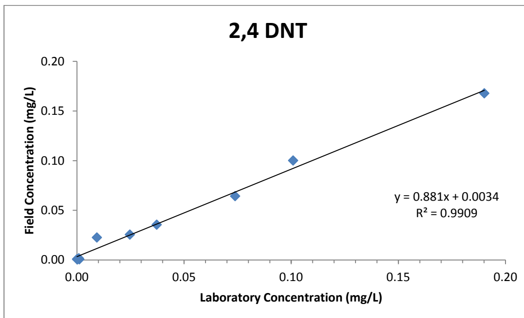
Figure 5.4. Griffin 450 field-analyzed data vs. traditional laboratory analysis by HPLC for 2,4-DNT.
