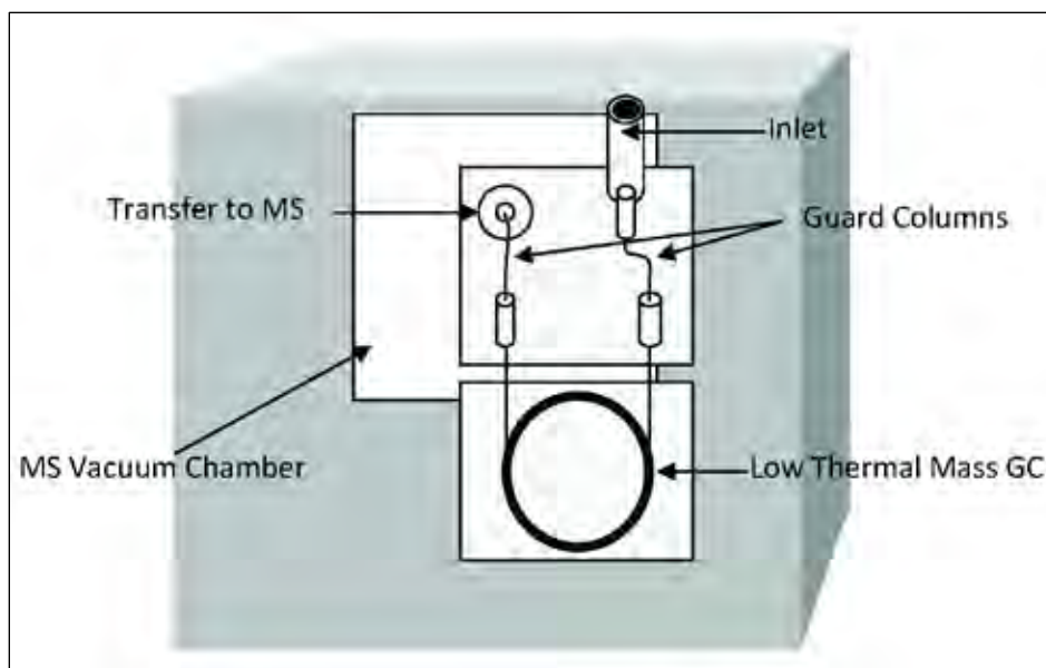
Figure 2.1. Components of the Griffin 450 GC-MS.
