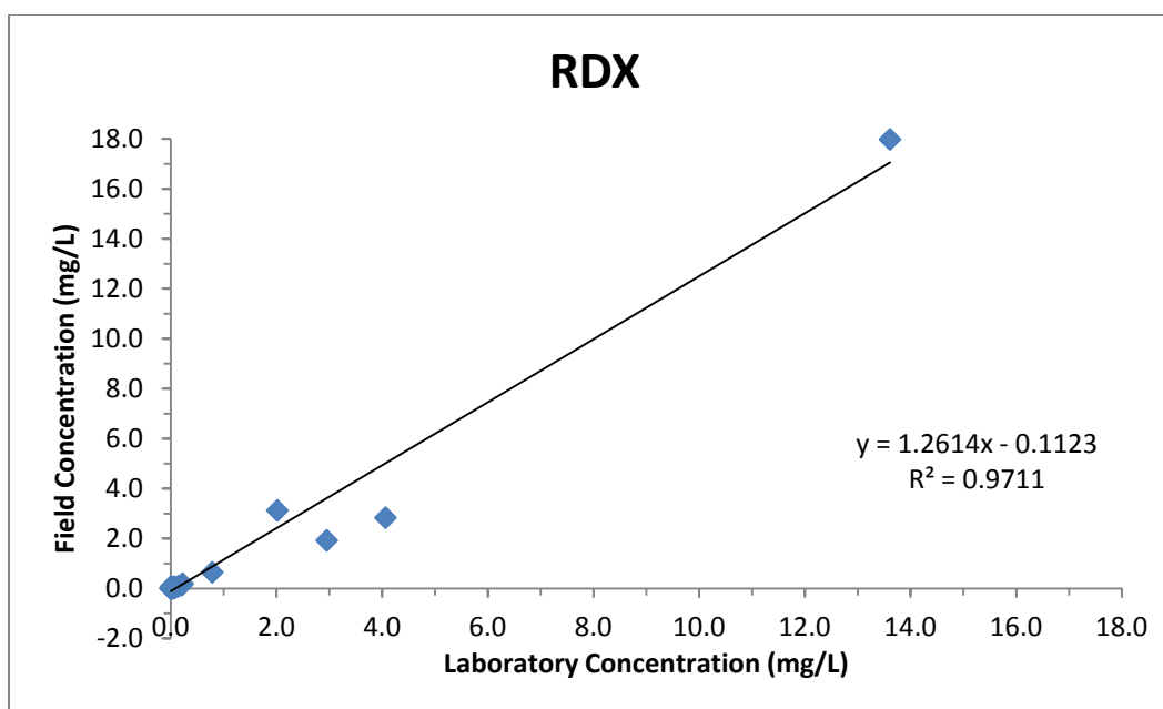
Figure 5.7. Griffin 450 field-analyzed data vs. traditional laboratory analysis by HPLC for RDX.
