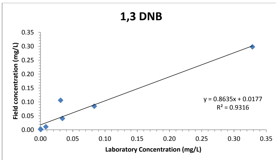
Figure 5.3. Griffin 450 field-analyzed data vs. traditional laboratory analysis by HPLC for 1,3-DNB.
