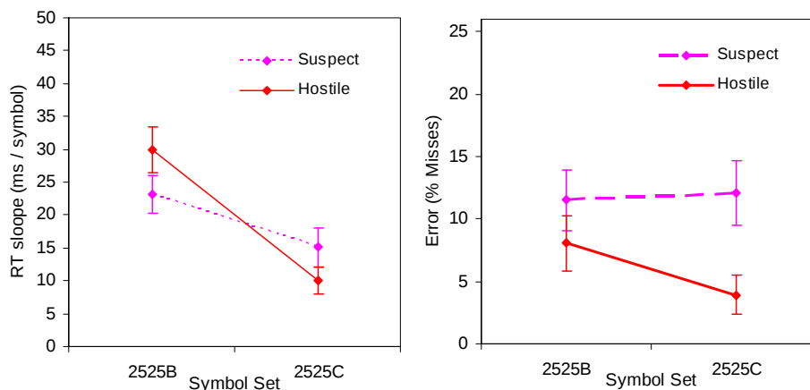
Figure 6 Mean RT Slope (left plot) and error (right plot) for the MIL-STD-2525B and MIL-STD-2525C representations of suspect and hostile affiliations. Error bars represent the 95 th percentile confidence intervals.
