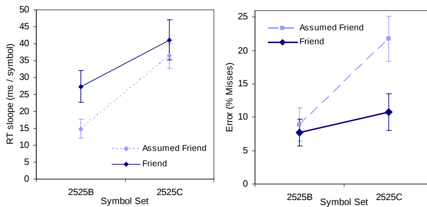
Figure 5 Mean RT Slope (left plot) and error (right plot) for the MIL-STD-2525B and MIL-STD-2525C representations of assumed friend and friend affiliations. Error bars represent the 95 th percentile confidence intervals.
