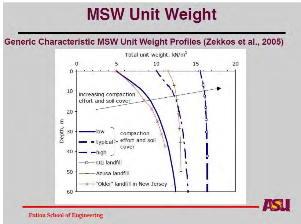
Figure 1: MSW Unit Weight Profile 3
