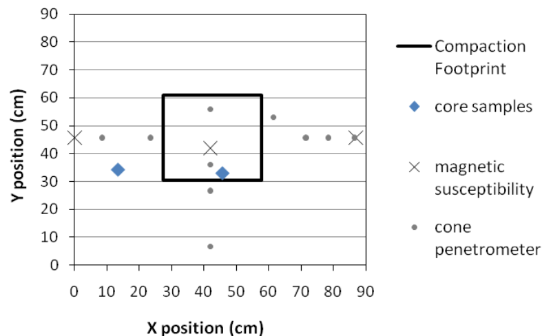
Figure 43. Relative Positions of Data Collection Locations for the Field Compaction Test 1. North is up.
