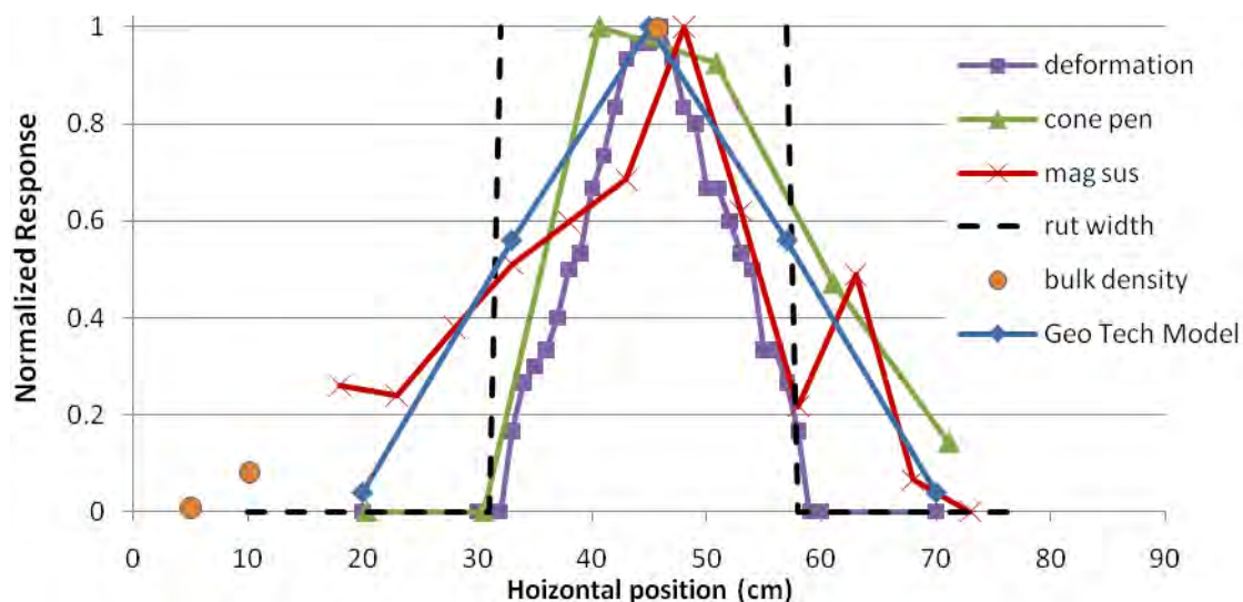
Figure 26. Normalized Results Laterally Across the Test Cell for Box Test 1. These data are from nominally 20 cm below the initial soil surface.
