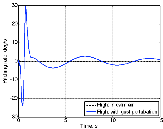
Figure 26. Pitching rate.
