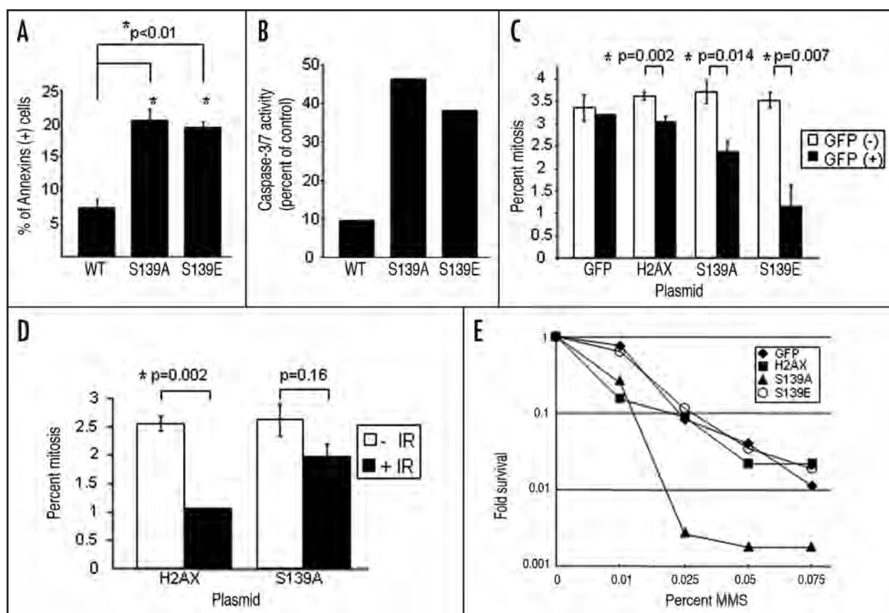
Figure 6. Effects of H2AX mutants on apoptosis and cell cycle checkpoints. (A) HeLa cells were transfected with GFP-H2AX, S139A or S139E and the percent increase of Annexin-V positive cells in the GFP positive cell population compared to the GFP negative cells in each sample was calculated. (B) HeLa cells were analyzed for caspase-3/7 activity 24 hours after transfection of H2AX, S139A, or the S139E constructs. Activity is relative to mock-transfected control cells. (C) Expression of S139E mutant triggers G 2 /M arrest in the absence of DNA damage. 293T cells were transfected with GFP, the GFP Vector, GFP-H2AX, S139A or S139E for 48 hours, and the percentage of cells in mitosis was quantified by phosphorylated histone H3 (Serine 10) by flow cytometry. Comparisons of the percentage of mitotic cells between GFP Negative and GFP Positive cells were made. (D) Expression of S139A mutant abrogates the ionizing radiation-induced G 2 /M arrest. 293T cells were transfected with the indicated constructs, irradiated with 6 Gy and analyzed one hour post-irradiation for phosphorylated histone H3. (E) Stable cell lines were treated with increasing doses of MMS for 50 minutes. Viability after 48 hours was measured by trypan blue exclusion.
