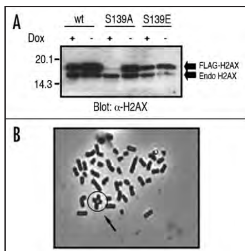
Figure 5. Induction of chromosome abnormalities in cells expressing H2AX S139A. (A) HCT116 Tet-off clones of cells expressing inducible FLAG-H2AX or mutants in the presence or absence of doxycycline (Dox). (B) Chromosome spreads showing a chromosomal aberration (red circle, black arrow), a quadriradial, found in cells expressing H2AX S139A.
