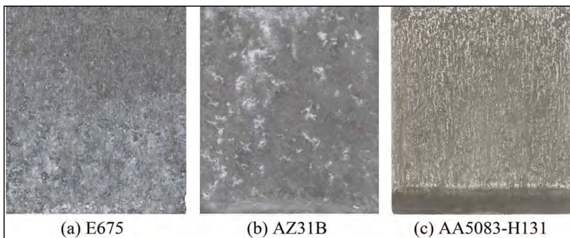
Figure 10. GM 9540P corrosion comparisons between armor plate alloys at 10 cycles.
