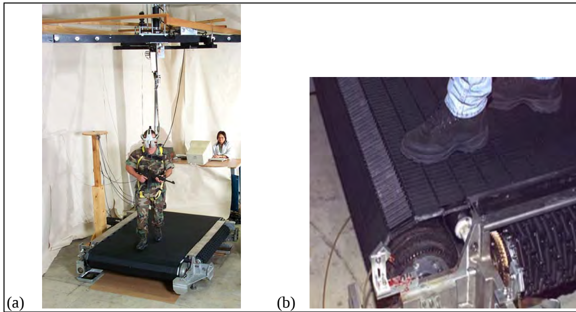
Figure 1. First-generation ODT (a) and first-generation ODT belt configuration (b).
