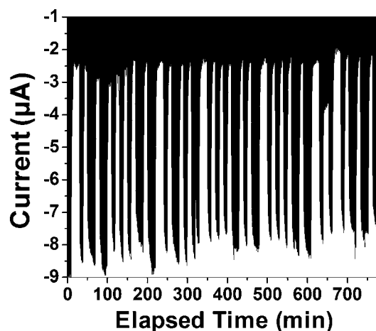
Fig. 3 Generation of a barcode from direct amperometric output of immobilized laccase. Input of N 2 - or O 2 -saturated electrolytes generates an amperometric output which can be programmed to yield a specific barcode by varying the residence time as demonstrated for the word “TEST”. Note: The figure can be directly read using a conventional barcode scanner.
