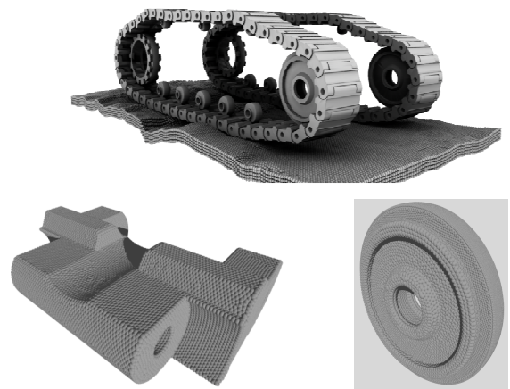
Figure 9: Snapshot from simulation of tracked vehicle on granular terrain (top), and examples of sphere-set collision geometry for two components of the track model (bottom).
