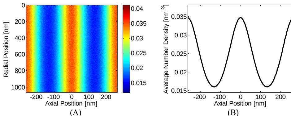
Figure 3 A) simulated number density [ \text{nm}^{-3} ] in 760 torr N_2 , and B) radially averaged value [ \text{nm}^{-3} ] of (A)
