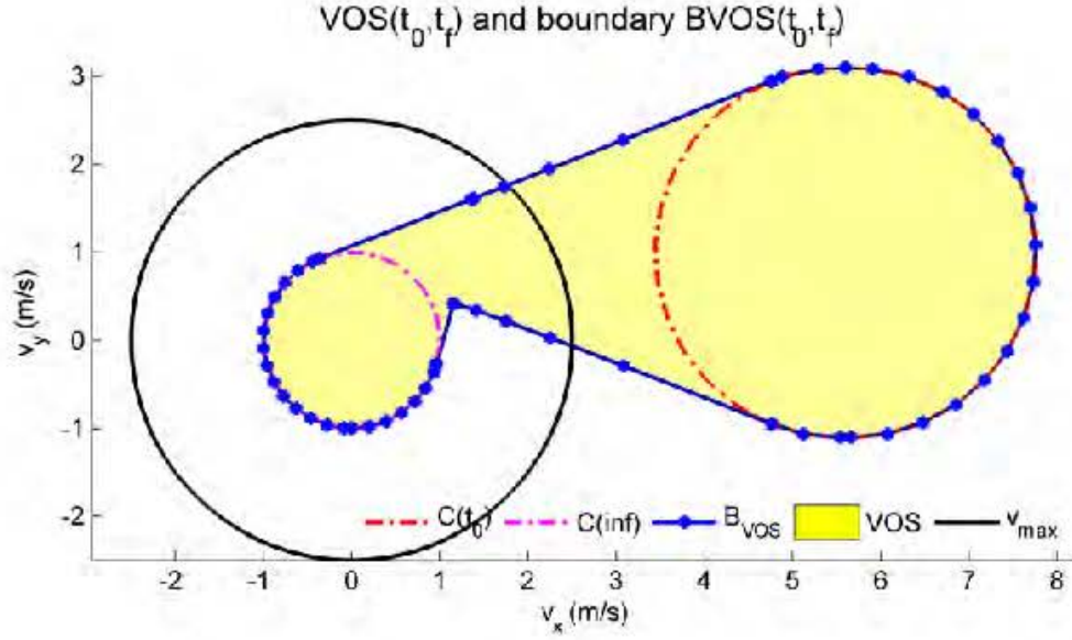
Figure 3-4: Velocity Obstacle Set for the same conditions. This set is computed using reachability. It always contains the region in Figure 3-3 as a subset; in this case they are identical if the region in Figure 3-3 were exhaustively defined.
