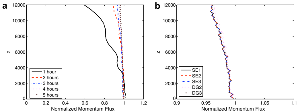
Fig. 13. Case 7: Linear Nonhydrostatic Mountain. Normalized momentum flux for 360 m (in x ) and 300 m (in z ) resolution and 10th order polynomials for (a) DG3 at times 1, 2, 3, 4, and 5 h, and (b) for all five models at 5 h.
