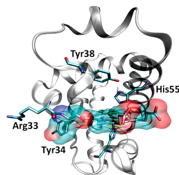
Figure 8. Selected residues in the heme environment of DHP. Tyr34, the site suggested to host the principal radical, is in van der Waals interaction with the heme porphyrin. Arg33 is in close proximity and might play a role in substrate binding. The pH 5 radical is proposed to be located on Tyr38, which can make a strong hydrogen bond with the distal His55. The PDB structure file 2QFK 10 was used to generate the figure.
