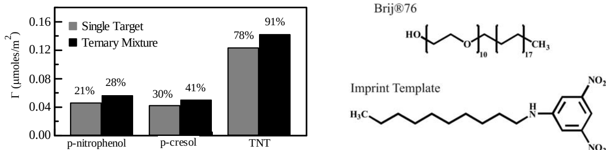
Figure 3. Adsorption of analytes by a molecularly-imprinted PMO from single target and ternary target solutions. \Gamma is the amount of target bound per unit surface area. Percentages are of the total target concentration in the sample. Also shown are the structure of Brij®76 and the imprint template molecule used.
