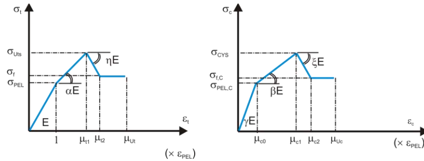
Fig. 1 Bilinear ascending curve and strain softening post peak response in tension and compression
