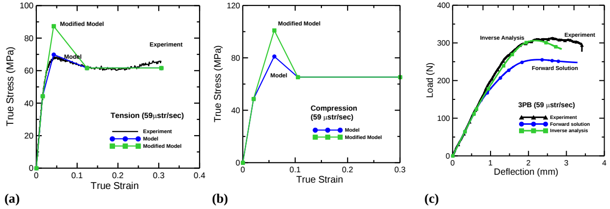
Fig. 13 Experiment and simulation of tension, compression and load deflection response at 59 \mu\text{str/sec}
