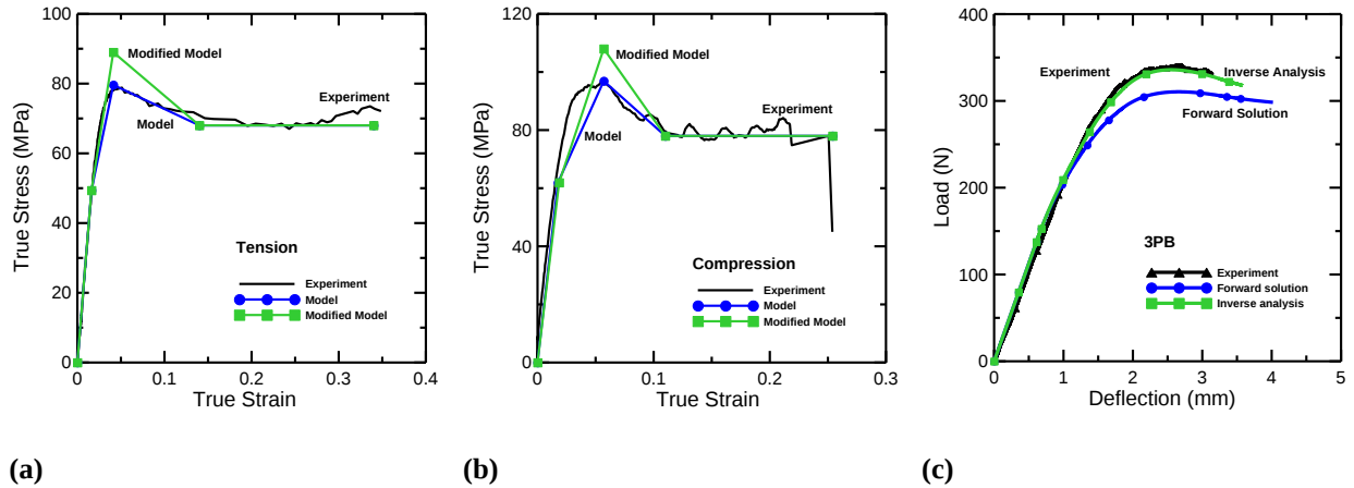
Fig. 12 Experiment and simulation of tension, compression and load deflection response at 493 \mu\text{str/sec}
